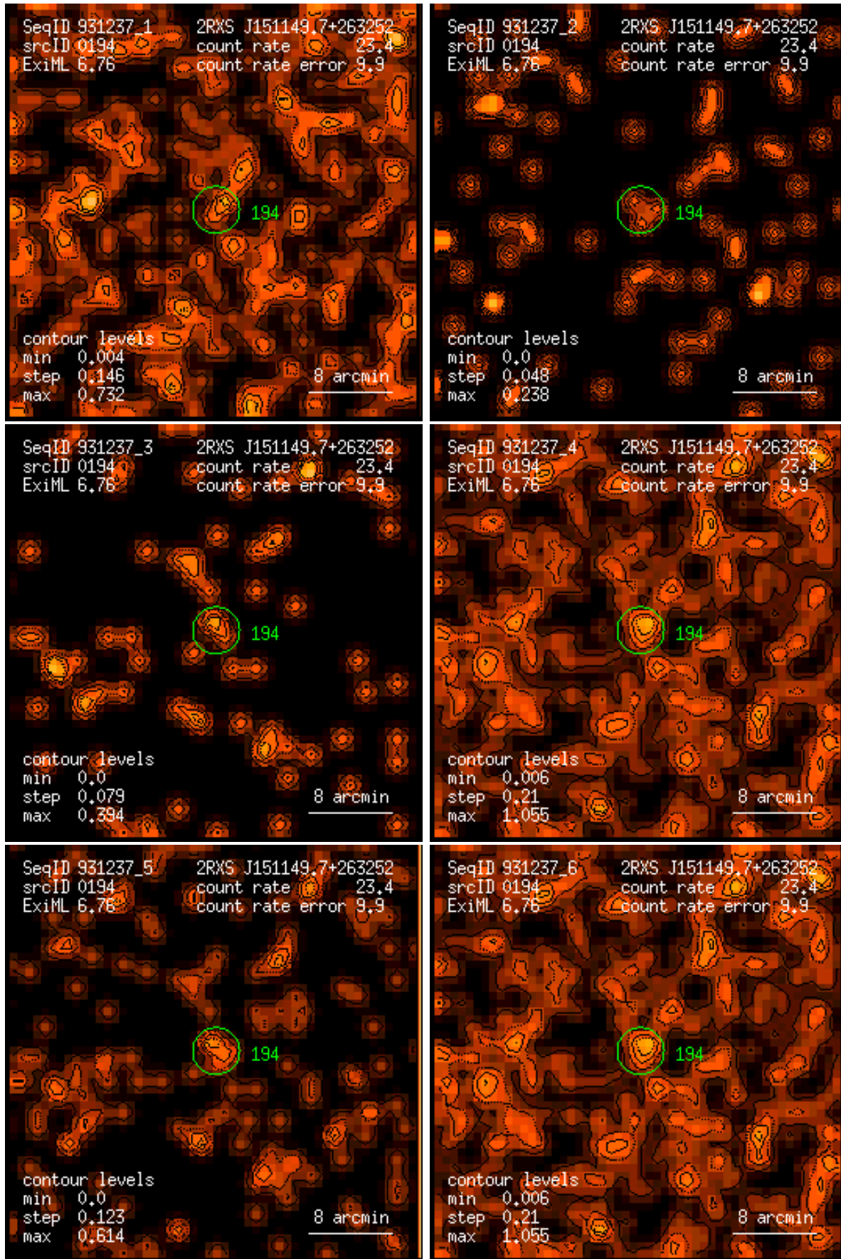
Figure 194: RASS 931237: detection 0194: band rate images, Gaussian filter: (1) PSPC channels 11 – 41, (2) 52 – 90, (3) 91 – 201, (4) 11 – 235, (5) 52 – 201, (6) 11 – 201. Broad band rates in counts/ks. Band rate contour levels in counts/ks/arcmin 2 .
