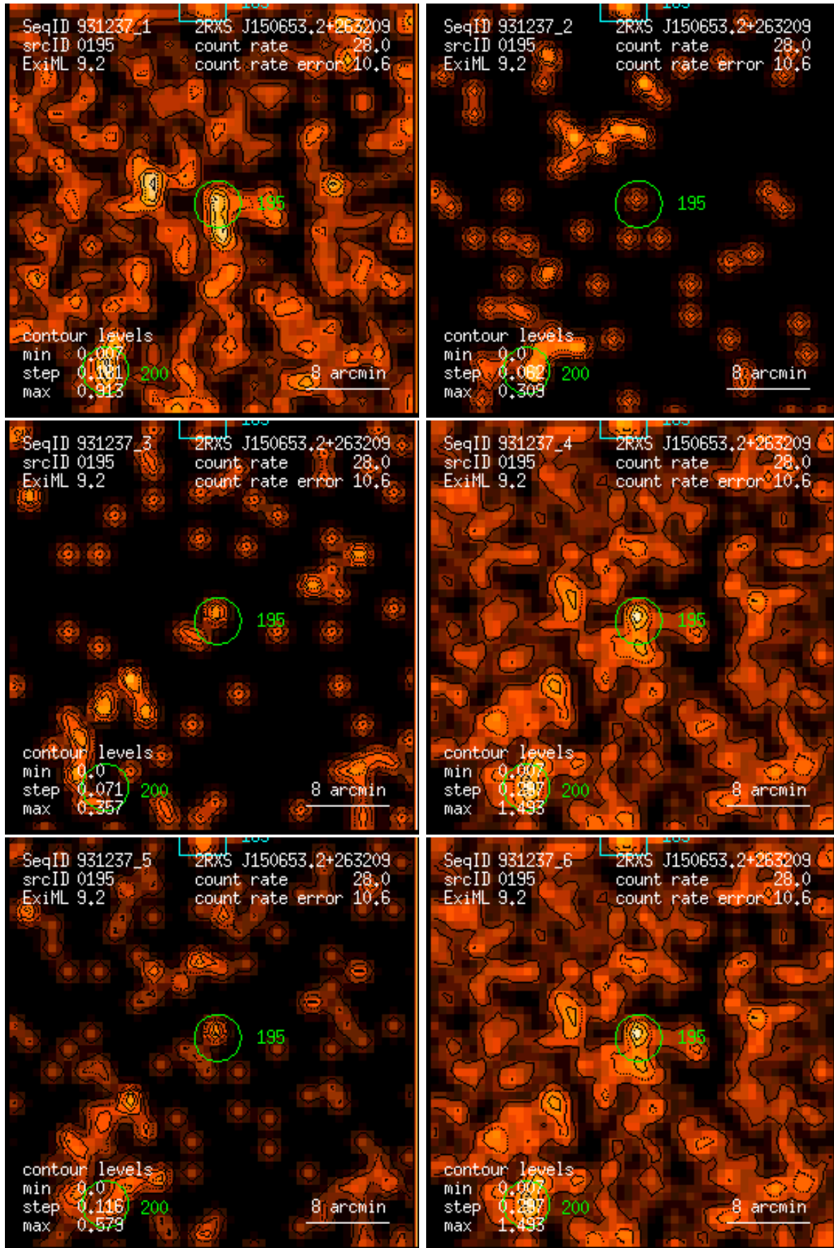
Figure 195: RASS 931237: detection 0195: band rate images, Gaussian filter: (1) PSPC channels 11 – 41, (2) 52 – 90, (3) 91 – 201, (4) 11 – 235, (5) 52 – 201, (6) 11 – 201. Broad band rates in counts/ks. Band rate contour levels in counts/ks/arcmin 2 .
