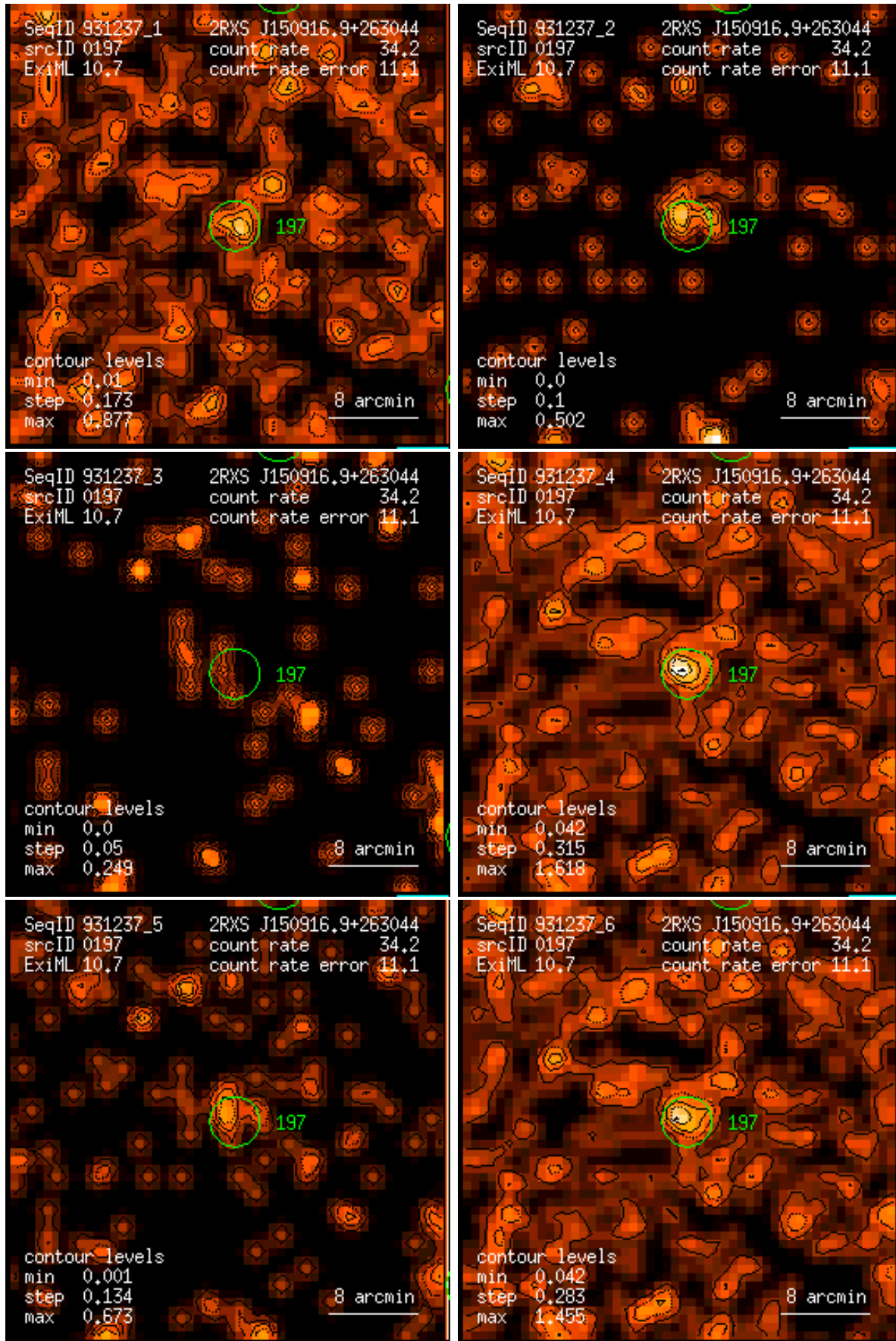
Figure 197: RASS 931237: detection 0197: band rate images, Gaussian filter: (1) PSPC channels 11 – 41, (2) 52 – 90, (3) 91 – 201, (4) 11 – 235, (5) 52 – 201, (6) 11 – 201. Broad band rates in counts/ks. Band rate contour levels in counts/ks/arcmin 2 .
