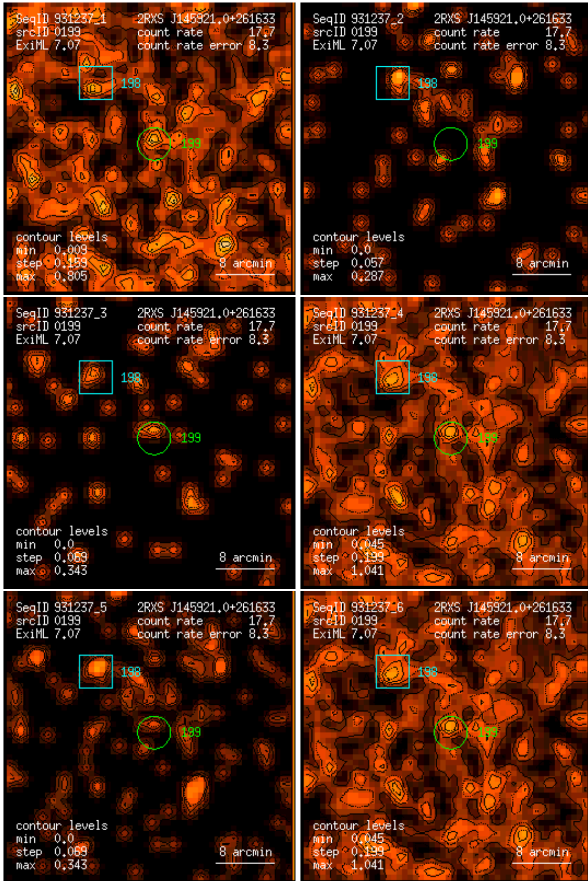
Figure 199: RASS 931237: detection 0199: band rate images, Gaussian filter: (1) PSPC channels 11 – 41, (2) 52 – 90, (3) 91 – 201, (4) 11 – 235, (5) 52 – 201, (6) 11 – 201. Broad band rates in counts/ks. Band rate contour levels in counts/ks/arcmin 2 .
