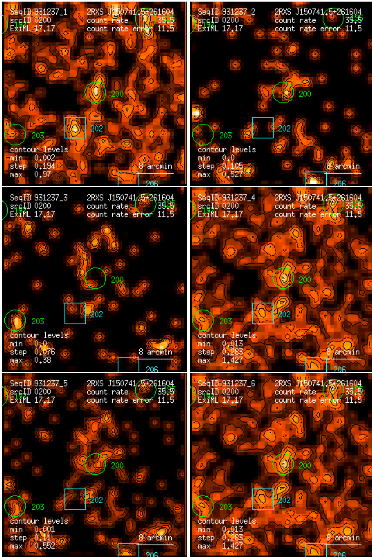
Figure 200: RASS 931237: detection 0200: band rate images, Gaussian filter: (1) PSPC channels 11 – 41, (2) 52 – 90, (3) 91 – 201, (4) 11 – 235, (5) 52 – 201, (6) 11 – 201. Broad band rates in counts/ks. Band rate contour levels in counts/ks/arcmin 2 .
