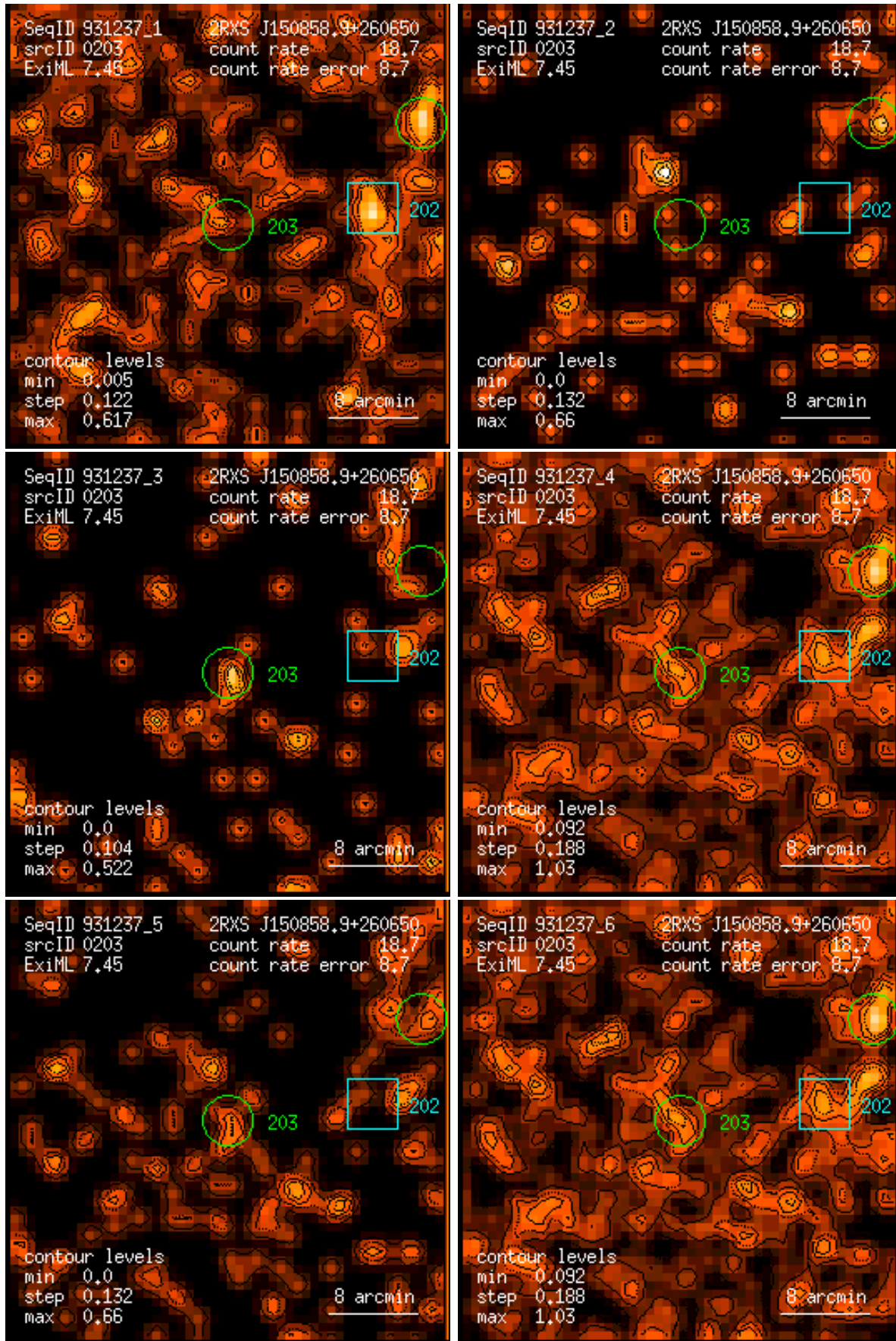
Figure 203: RASS 931237: detection 0203: band rate images, Gaussian filter: (1) PSPC channels 11 – 41, (2) 52 – 90, (3) 91 – 201, (4) 11 – 235, (5) 52 – 201, (6) 11 – 201. Broad band rates in counts/ks. Band rate contour levels in counts/ks/arcmin 2 .
