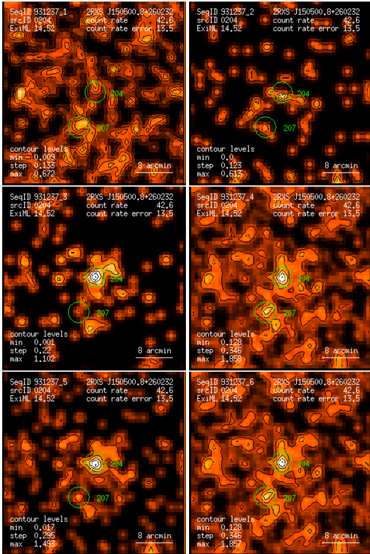
Figure 204: RASS 931237: detection 0204: band rate images, Gaussian filter: (1) PSPC channels 11 – 41, (2) 52 – 90, (3) 91 – 201, (4) 11 – 235, (5) 52 – 201, (6) 11 – 201. Broad band rates in counts/ks. Band rate contour levels in counts/ks/arcmin 2 .
