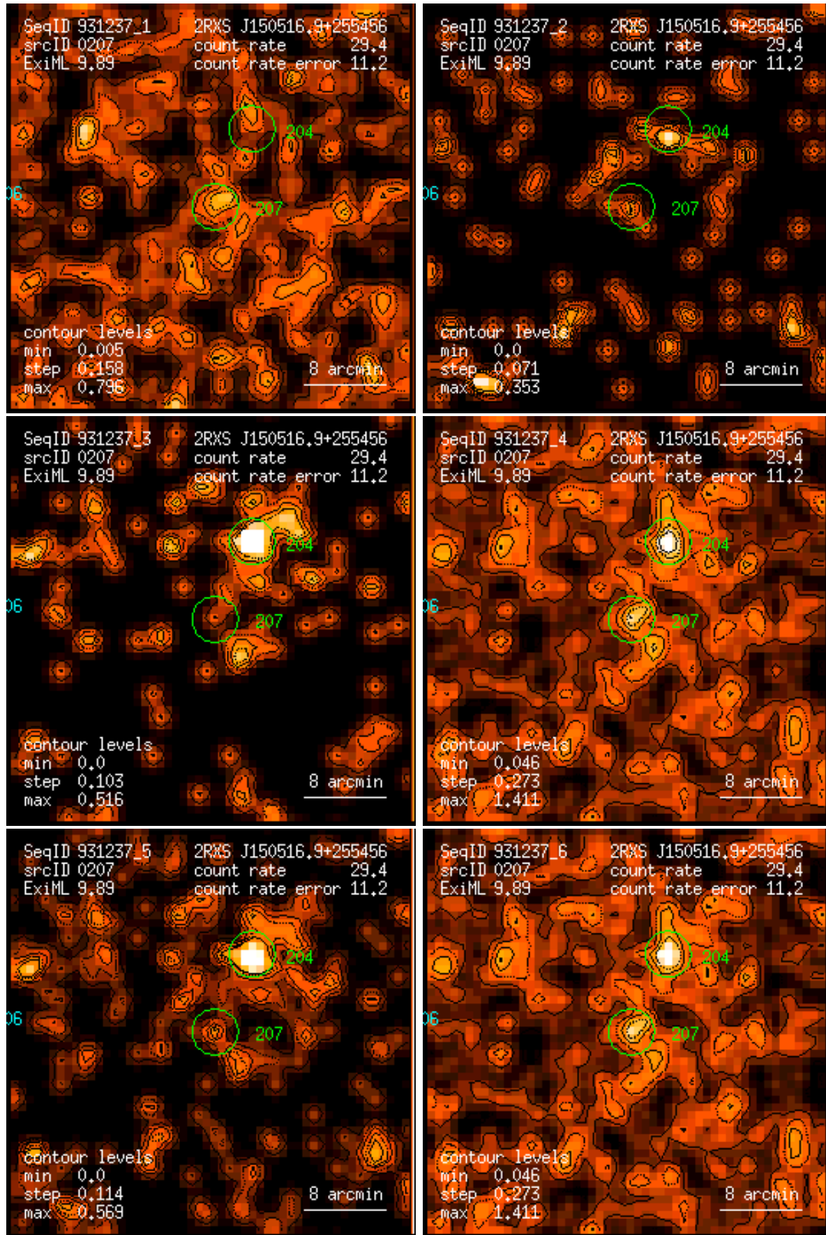
Figure 207: RASS 931237: detection 0207: band rate images, Gaussian filter: (1) PSPC channels 11 – 41, (2) 52 – 90, (3) 91 – 201, (4) 11 – 235, (5) 52 – 201, (6) 11 – 201. Broad band rates in counts/ks. Band rate contour levels in counts/ks/arcmin 2 .
