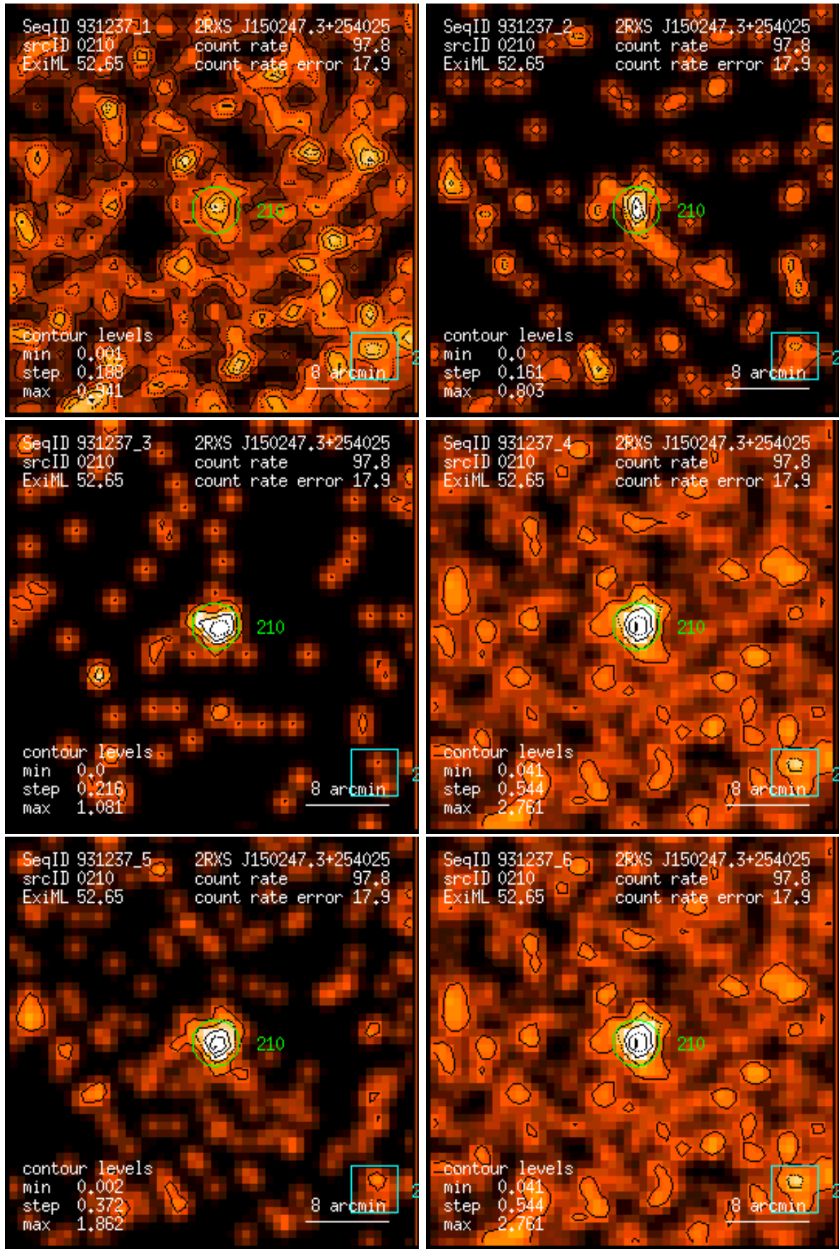
Figure 210: RASS 931237: detection 0210: band rate images, Gaussian filter: (1) PSPC channels 11 – 41, (2) 52 – 90, (3) 91 – 201, (4) 11 – 235, (5) 52 – 201, (6) 11 – 201. Broad band rates in counts/ks. Band rate contour levels in counts/ks/arcmin 2 .
