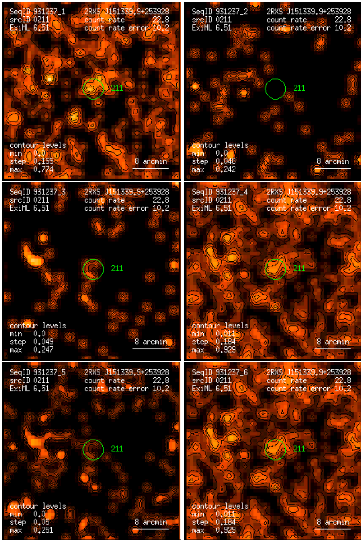
Figure 211: RASS 931237: detection 0211: band rate images, Gaussian filter: (1) PSPC channels 11 – 41, (2) 52 – 90, (3) 91 – 201, (4) 11 – 235, (5) 52 – 201, (6) 11 – 201. Broad band rates in counts/ks. Band rate contour levels in counts/ks/arcmin 2 .
