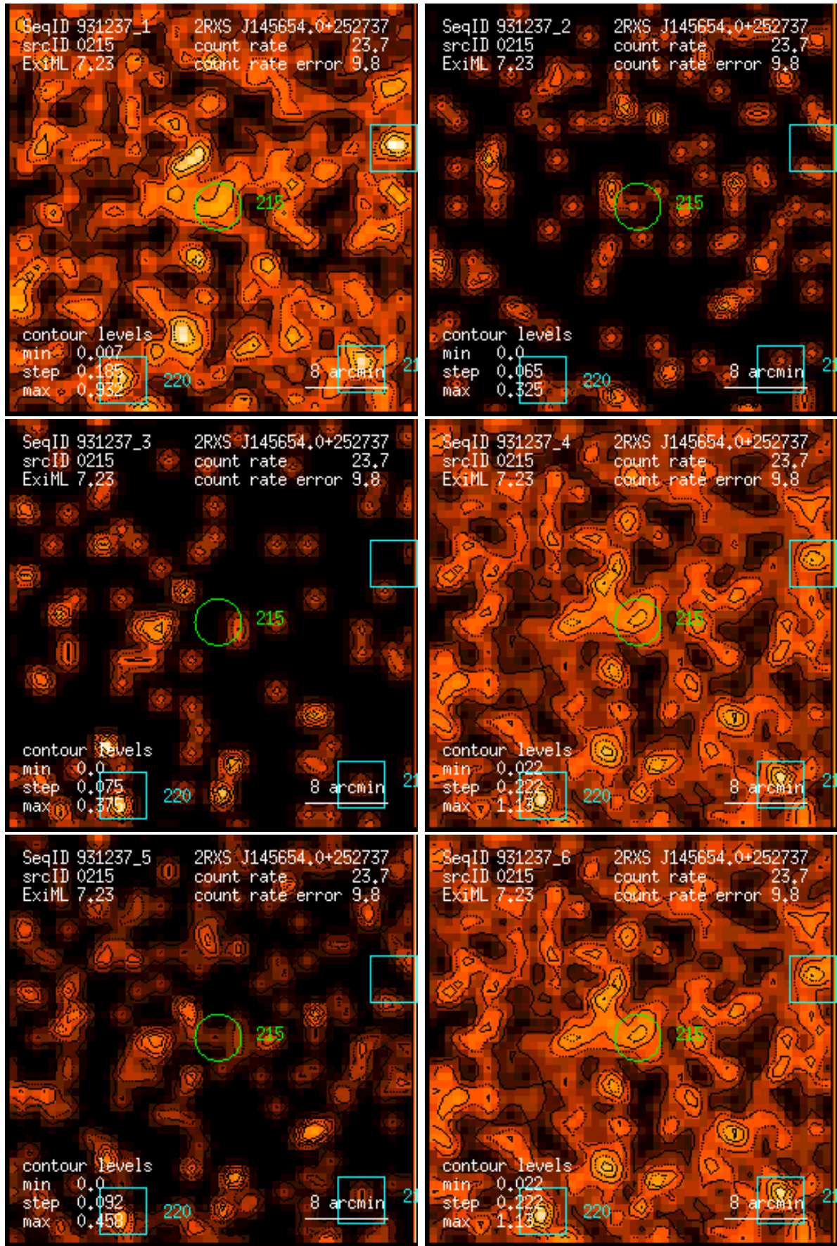
Figure 215: RASS 931237: detection 0215: band rate images, Gaussian filter: (1) PSPC channels 11 – 41, (2) 52 – 90, (3) 91 – 201, (4) 11 – 235, (5) 52 – 201, (6) 11 – 201. Broad band rates in counts/ks. Band rate contour levels in counts/ks/arcmin 2 .
