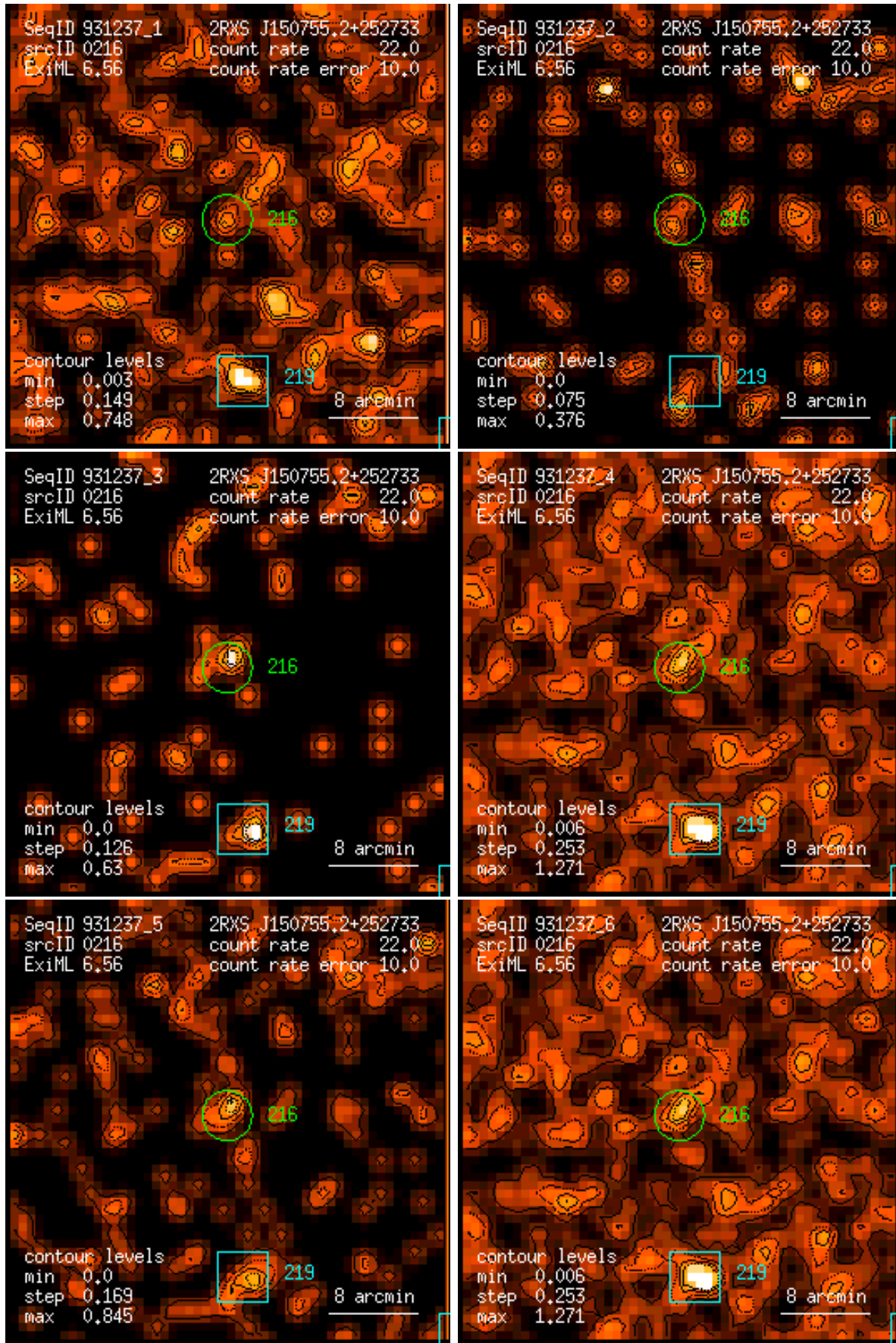
Figure 216: RASS 931237: detection 0216: band rate images, Gaussian filter: (1) PSPC channels 11 – 41, (2) 52 – 90, (3) 91 – 201, (4) 11 – 235, (5) 52 – 201, (6) 11 – 201. Broad band rates in counts/ks. Band rate contour levels in counts/ks/arcmin 2 .
