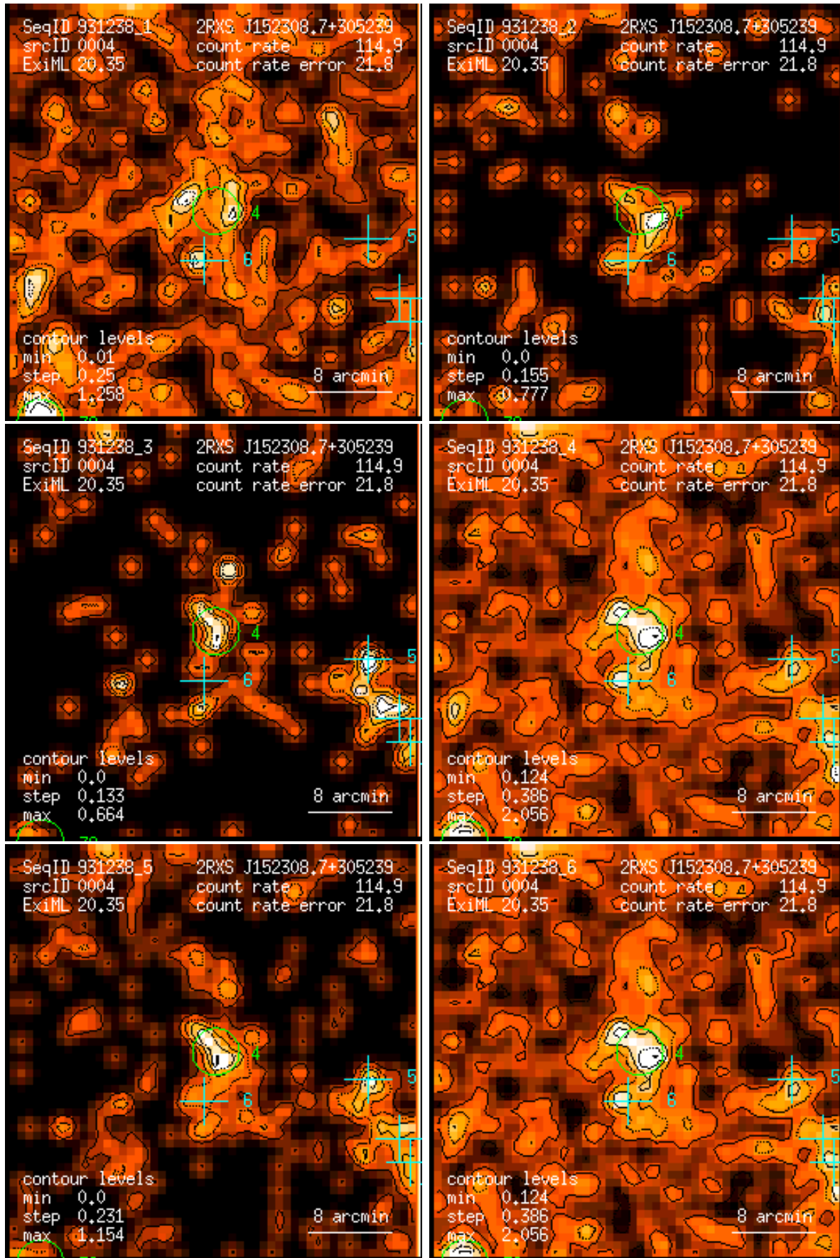
Figure 4: RASS 931238: detection 0004: band rate images, Gaussian filter: (1) PSPC channels 11 – 41, (2) 52 – 90, (3) 91 – 201, (4) 11 – 235, (5) 52 – 201, (6) 11 – 201. Broad band rates in counts/ks. Band rate contour levels in counts/ks/arcmin 2 .
