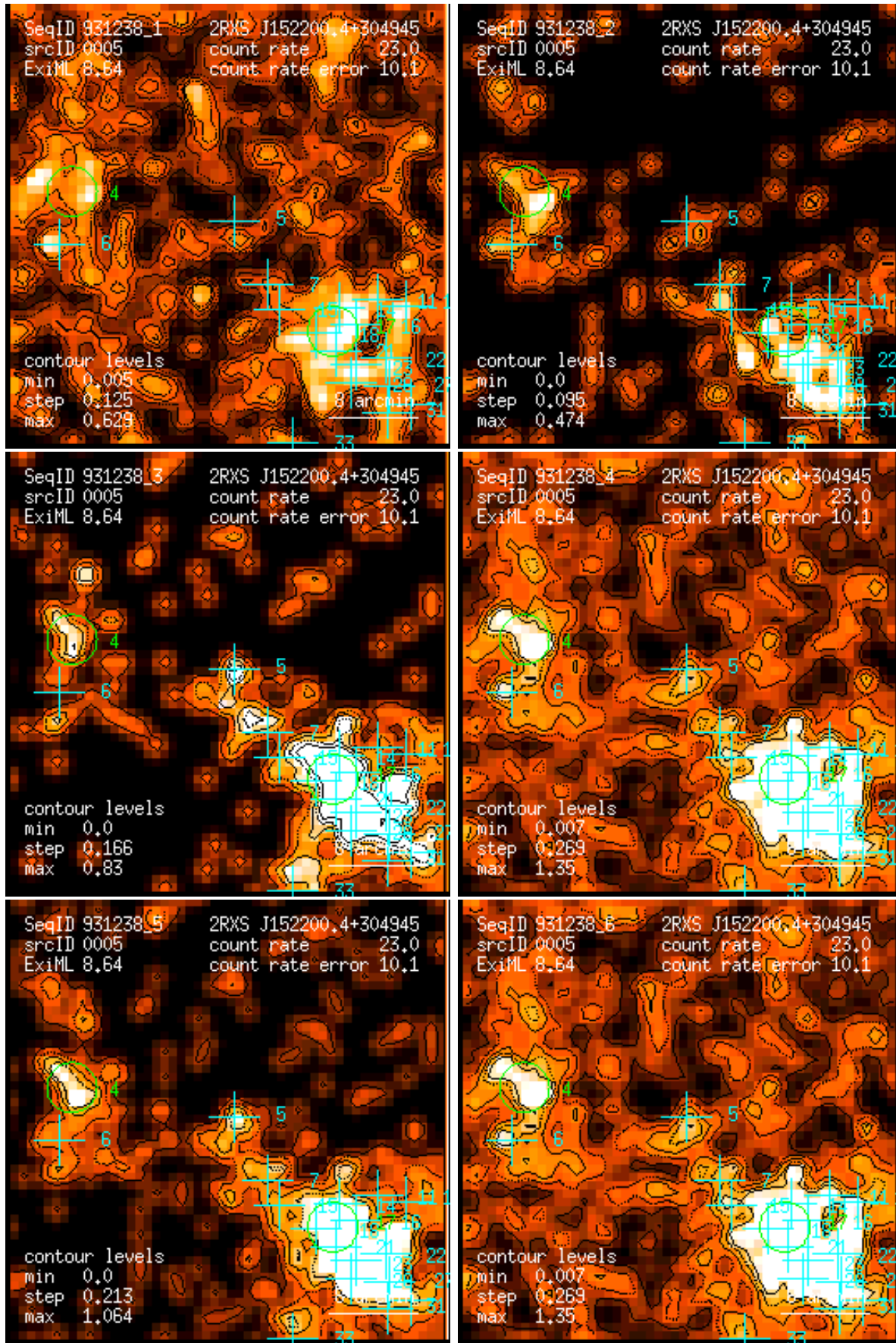
Figure 5: RASS 931238: detection 0005: band rate images, Gaussian filter: (1) PSPC channels 11 – 41, (2) 52 – 90, (3) 91 – 201, (4) 11 – 235, (5) 52 – 201, (6) 11 – 201. Broad band rates in counts/ks. Band rate contour levels in counts/ks/arcmin 2 .
