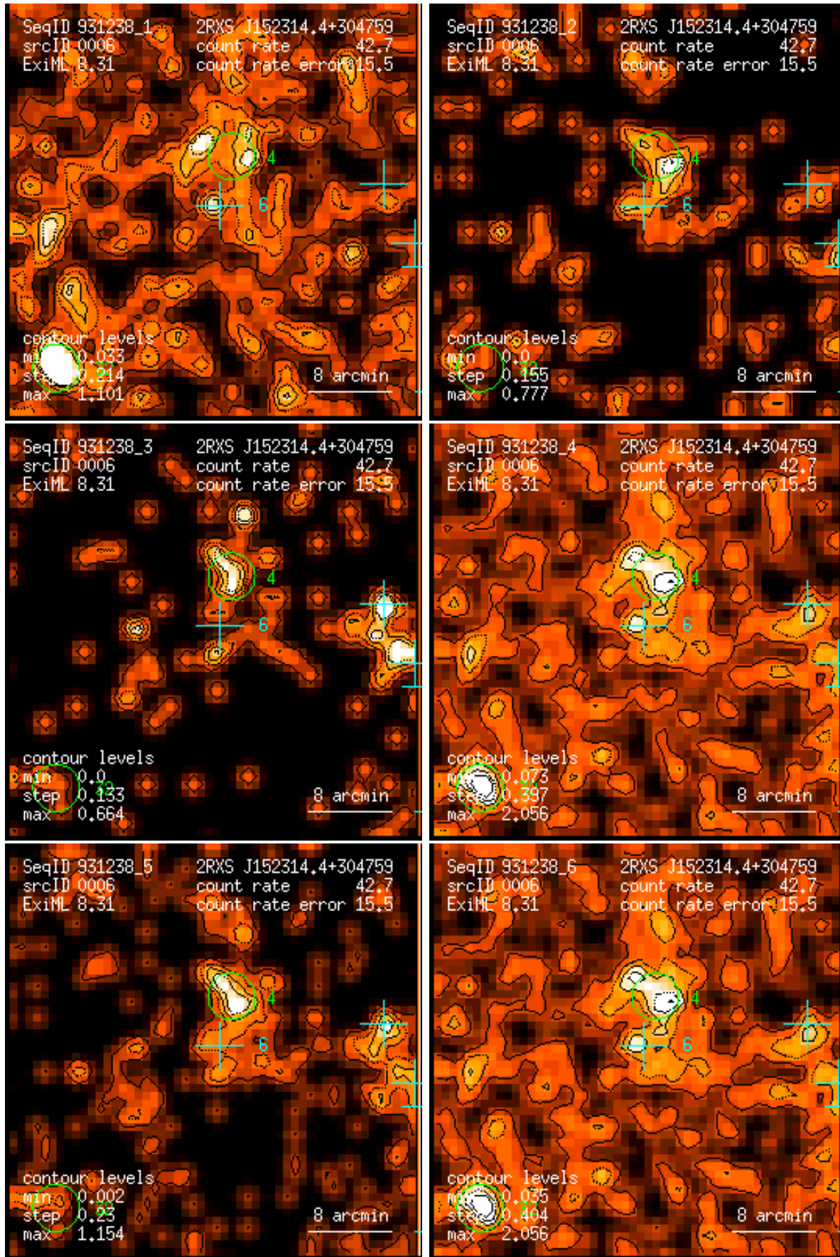
Figure 6: RASS 931238: detection 0006: band rate images, Gaussian filter: (1) PSPC channels 11 – 41, (2) 52 – 90, (3) 91 – 201, (4) 11 – 235, (5) 52 – 201, (6) 11 – 201. Broad band rates in counts/ks. Band rate contour levels in counts/ks/arcmin 2 .
