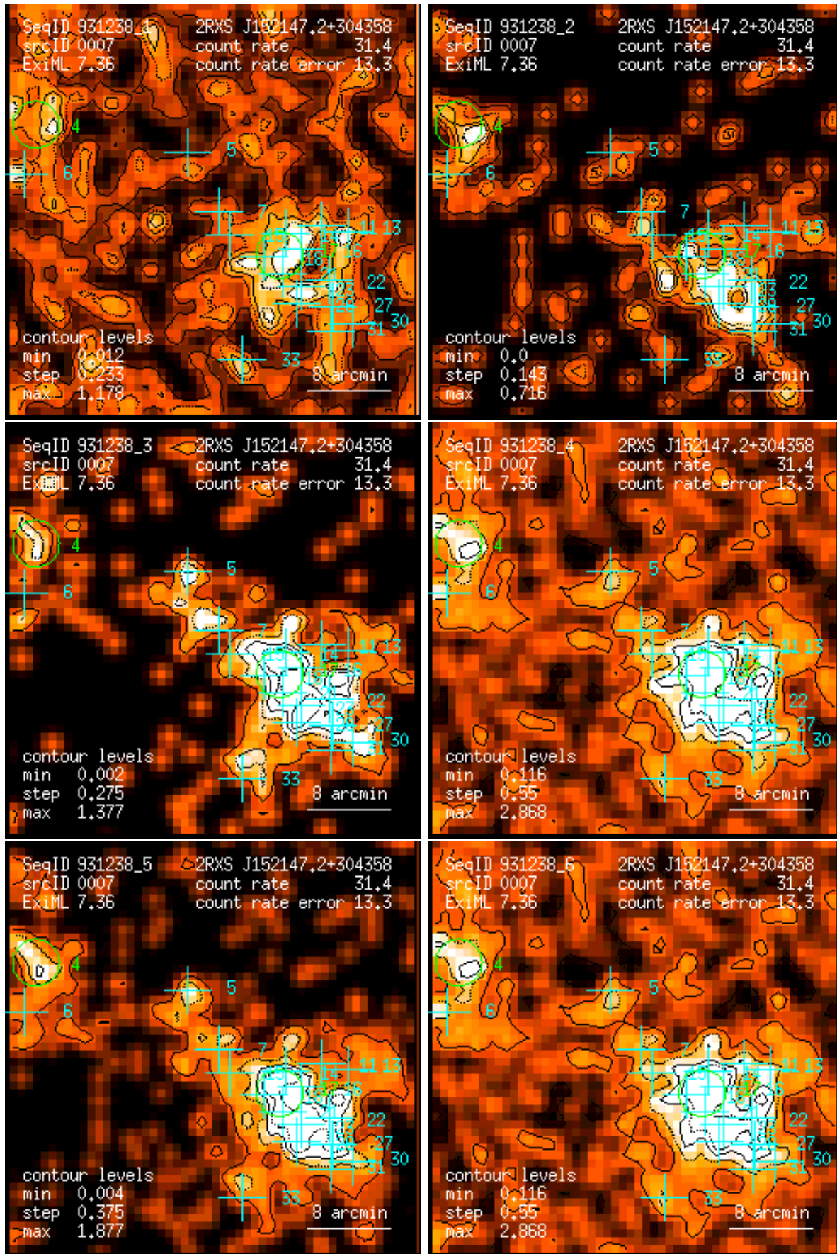
Figure 7: RASS 931238: detection 0007: band rate images, Gaussian filter: (1) PSPC channels 11 – 41, (2) 52 – 90, (3) 91 – 201, (4) 11 – 235, (5) 52 – 201, (6) 11 – 201. Broad band rates in counts/ks. Band rate contour levels in counts/ks/arcmin 2 .
