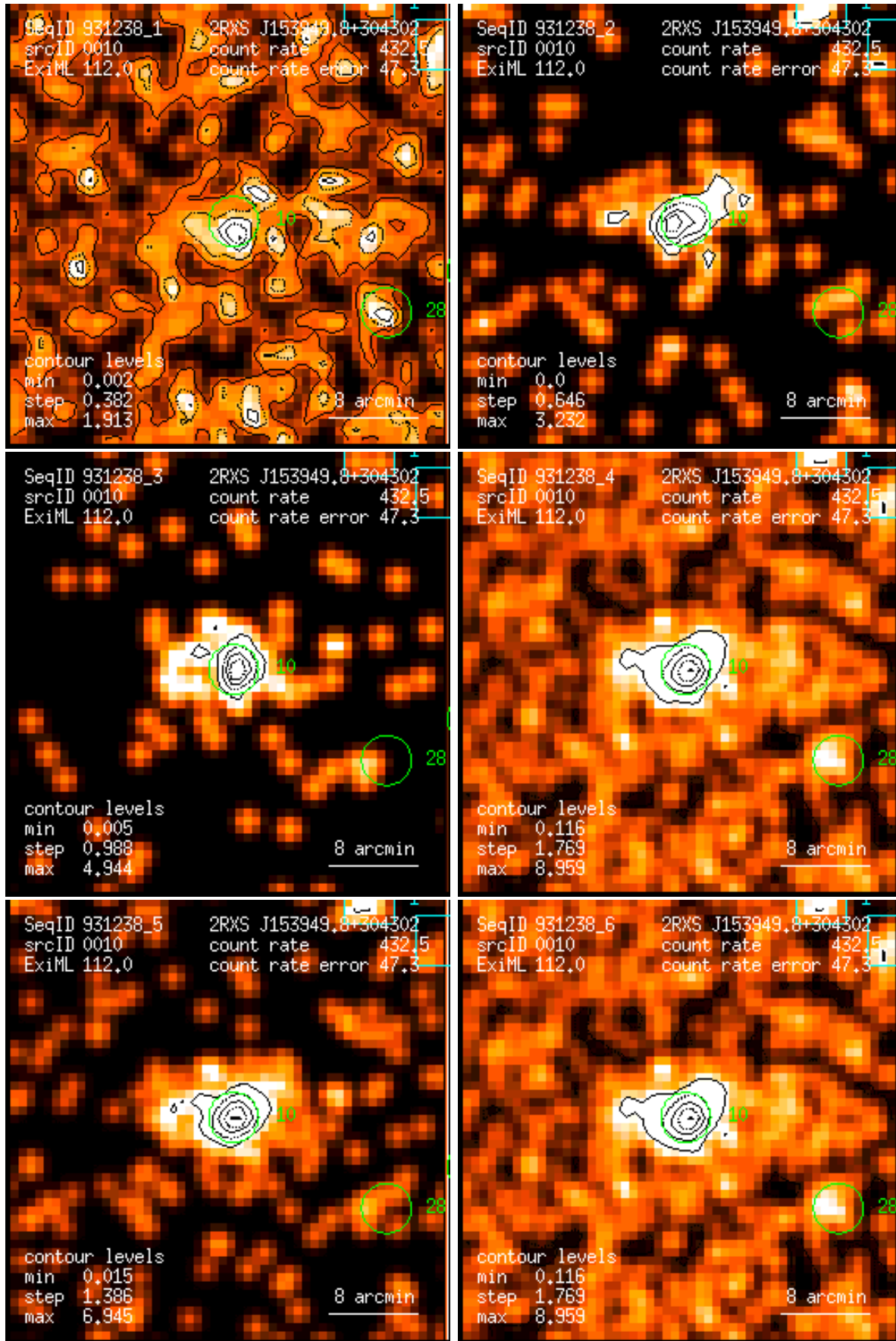
Figure 10: RASS 931238: detection 0010: band rate images, Gaussian filter: (1) PSPC channels 11 – 41, (2) 52 – 90, (3) 91 – 201, (4) 11 – 235, (5) 52 – 201, (6) 11 – 201. Broad band rates in counts/ks. Band rate contour levels in counts/ks/arcmin 2 .
