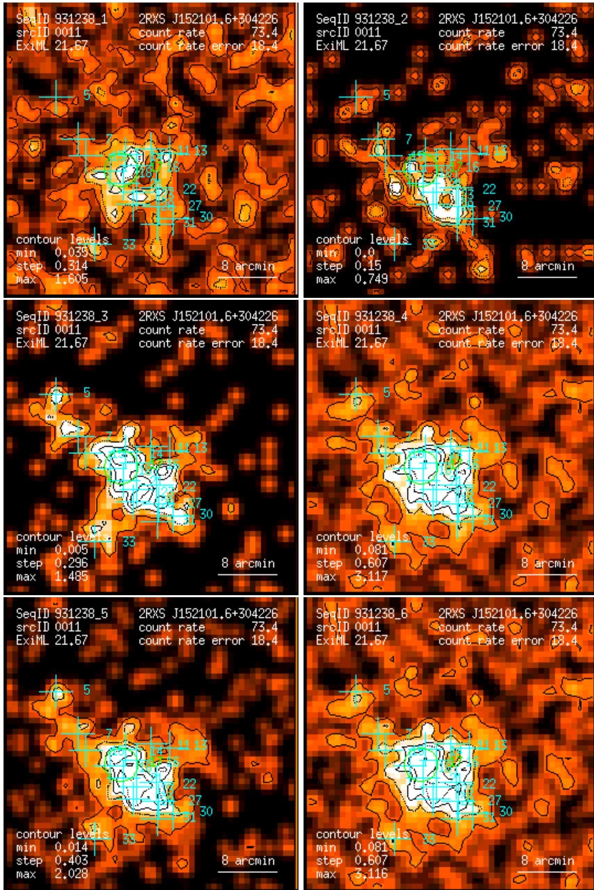
Figure 11: RASS 931238: detection 0011: band rate images, Gaussian filter: (1) PSPC channels 11 – 41, (2) 52 – 90, (3) 91 – 201, (4) 11 – 235, (5) 52 – 201, (6) 11 – 201. Broad band rates in counts/ks. Band rate contour levels in counts/ks/arcmin 2 .
