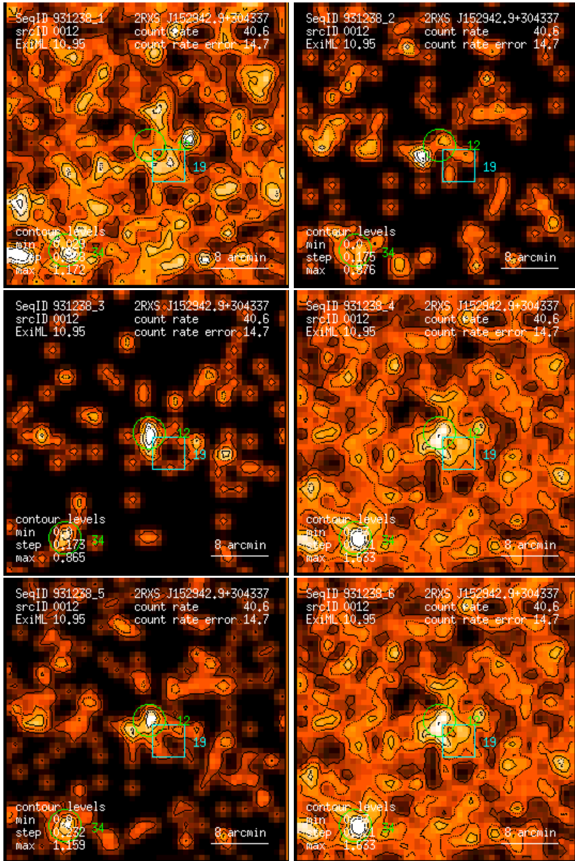
Figure 12: RASS 931238: detection 0012: band rate images, Gaussian filter: (1) PSPC channels 11 – 41, (2) 52 – 90, (3) 91 – 201, (4) 11 – 235, (5) 52 – 201, (6) 11 – 201. Broad band rates in counts/ks. Band rate contour levels in counts/ks/arcmin 2 .
