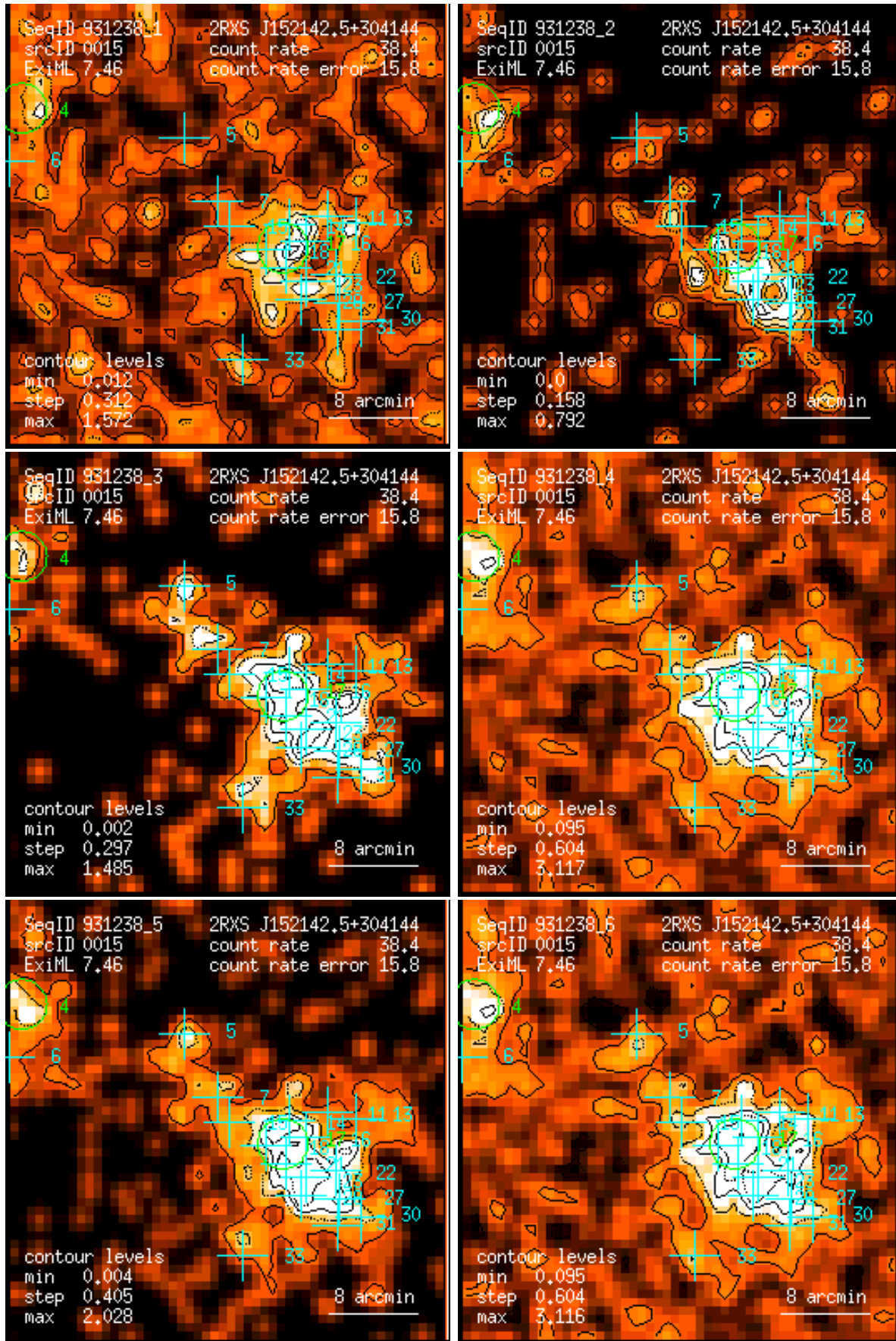
Figure 15: RASS 931238: detection 0015: band rate images, Gaussian filter: (1) PSPC channels 11 – 41, (2) 52 – 90, (3) 91 – 201, (4) 11 – 235, (5) 52 – 201, (6) 11 – 201. Broad band rates in counts/ks. Band rate contour levels in counts/ks/arcmin 2 .
