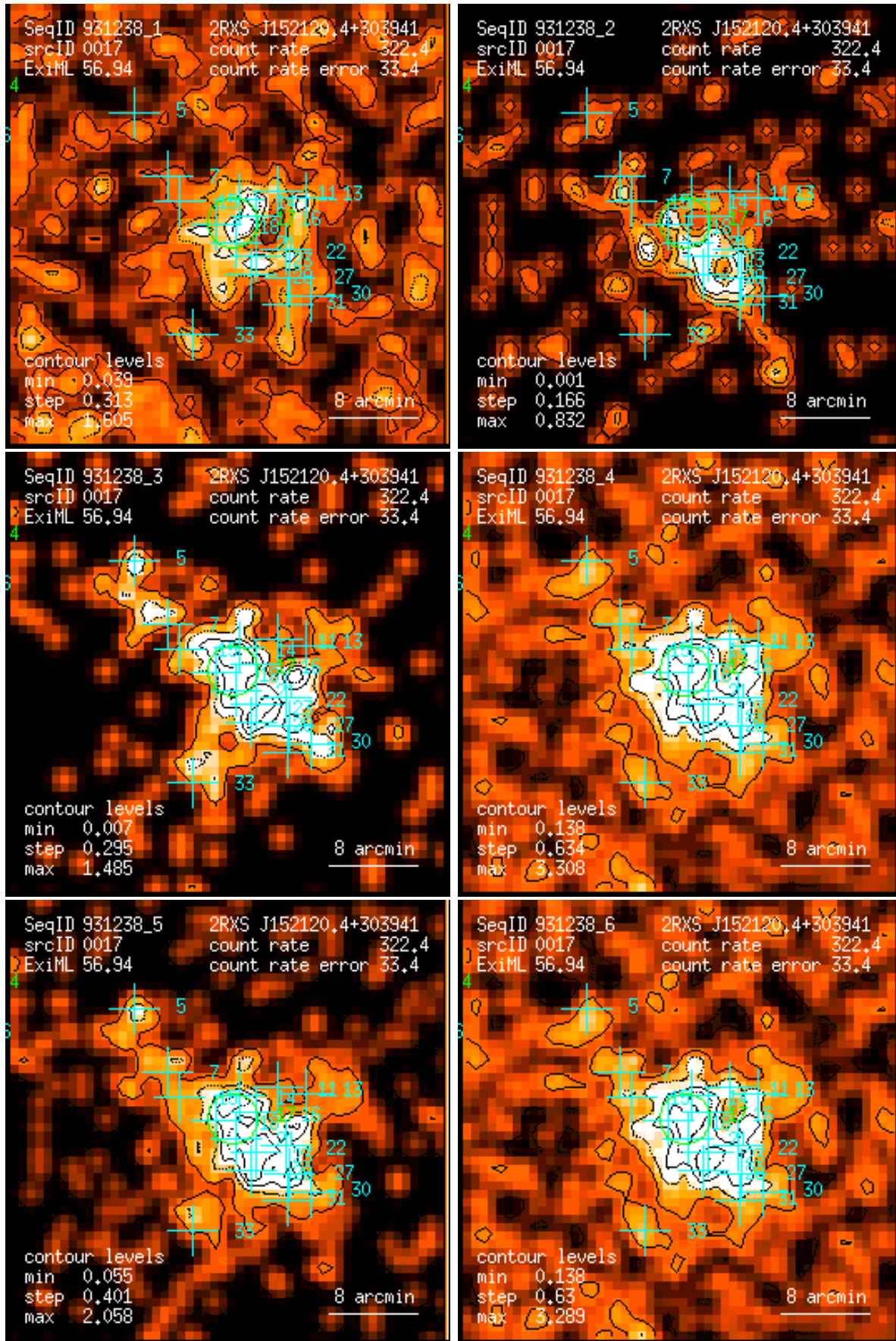
Figure 17: RASS 931238: detection 0017: band rate images, Gaussian filter: (1) PSPC channels 11 – 41, (2) 52 – 90, (3) 91 – 201, (4) 11 – 235, (5) 52 – 201, (6) 11 – 201. Broad band rates in counts/ks. Band rate contour levels in counts/ks/arcmin 2 .
