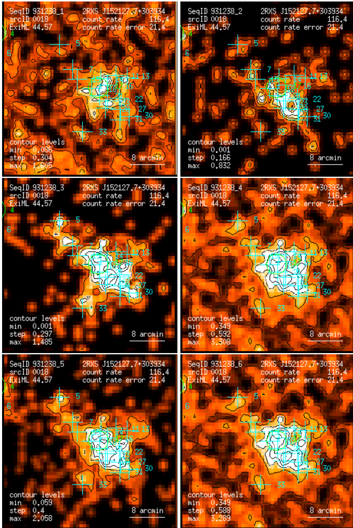
Figure 18: RASS 931238: detection 0018: band rate images, Gaussian filter: (1) PSPC channels 11 – 41, (2) 52 – 90, (3) 91 – 201, (4) 11 – 235, (5) 52 – 201, (6) 11 – 201. Broad band rates in counts/ks. Band rate contour levels in counts/ks/arcmin 2 .
