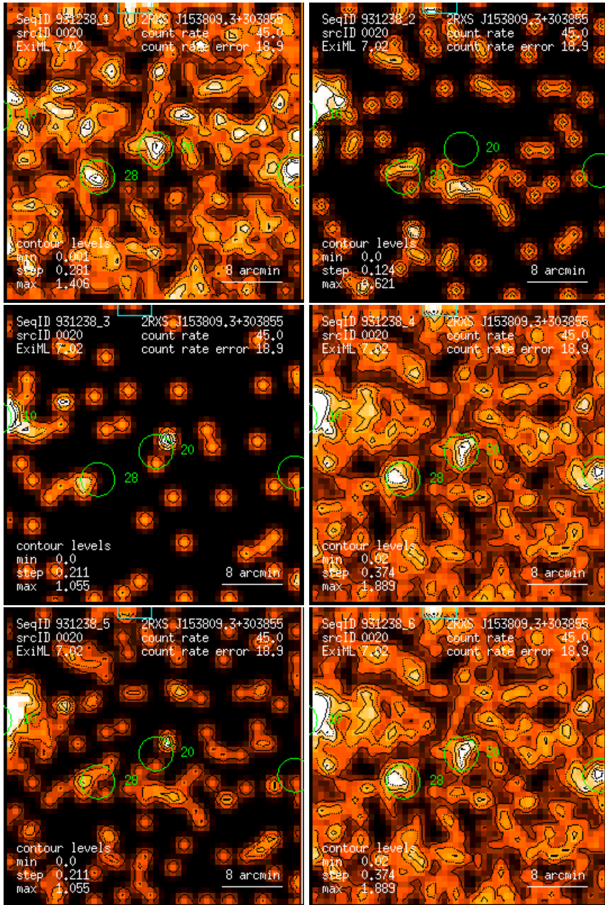
Figure 20: RASS 931238: detection 0020: band rate images, Gaussian filter: (1) PSPC channels 11 – 41, (2) 52 – 90, (3) 91 – 201, (4) 11 – 235, (5) 52 – 201, (6) 11 – 201. Broad band rates in counts/ks. Band rate contour levels in counts/ks/arcmin 2 .
