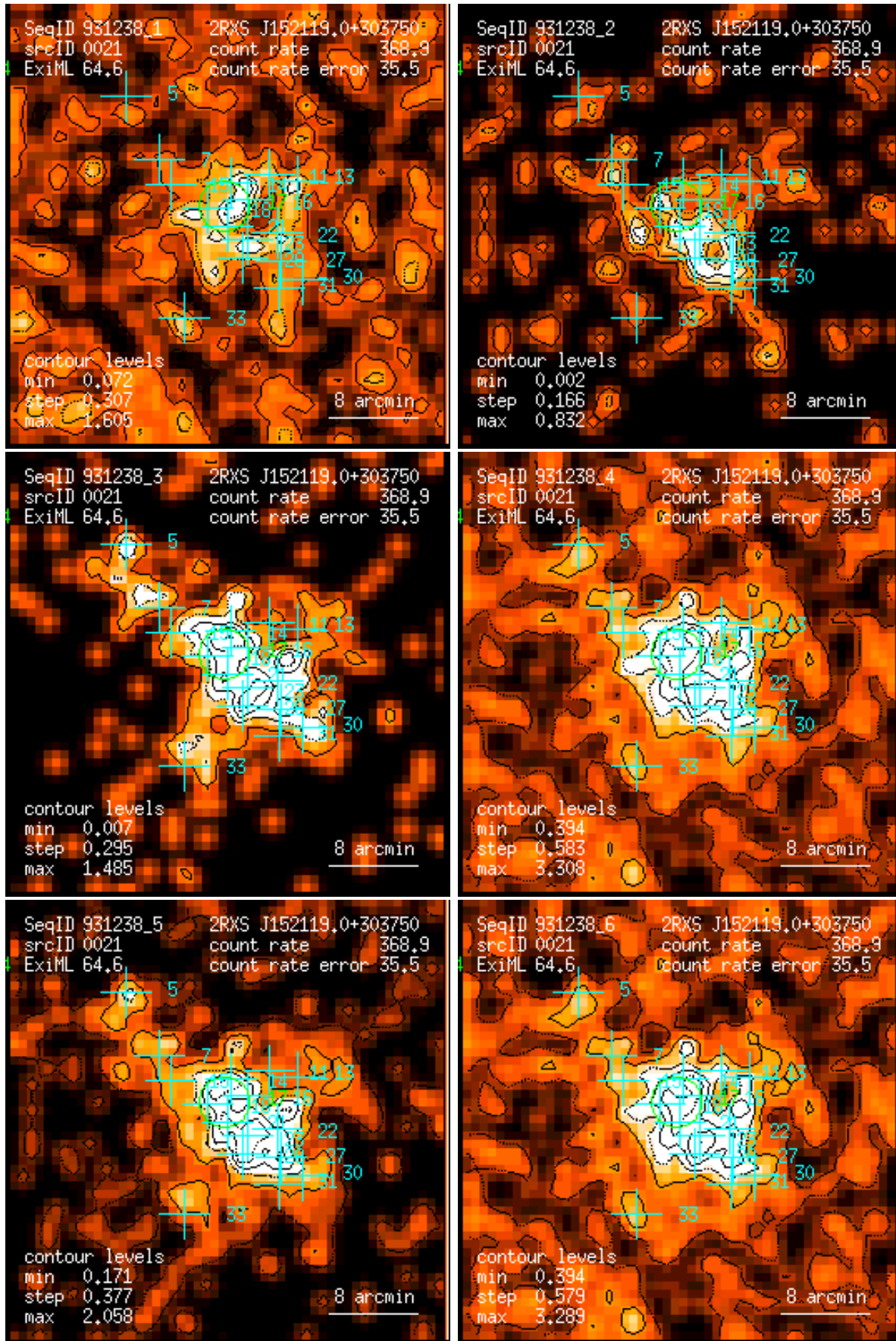
Figure 21: RASS 931238: detection 0021: band rate images, Gaussian filter: (1) PSPC channels 11 – 41, (2) 52 – 90, (3) 91 – 201, (4) 11 – 235, (5) 52 – 201, (6) 11 – 201. Broad band rates in counts/ks. Band rate contour levels in counts/ks/arcmin 2 .
