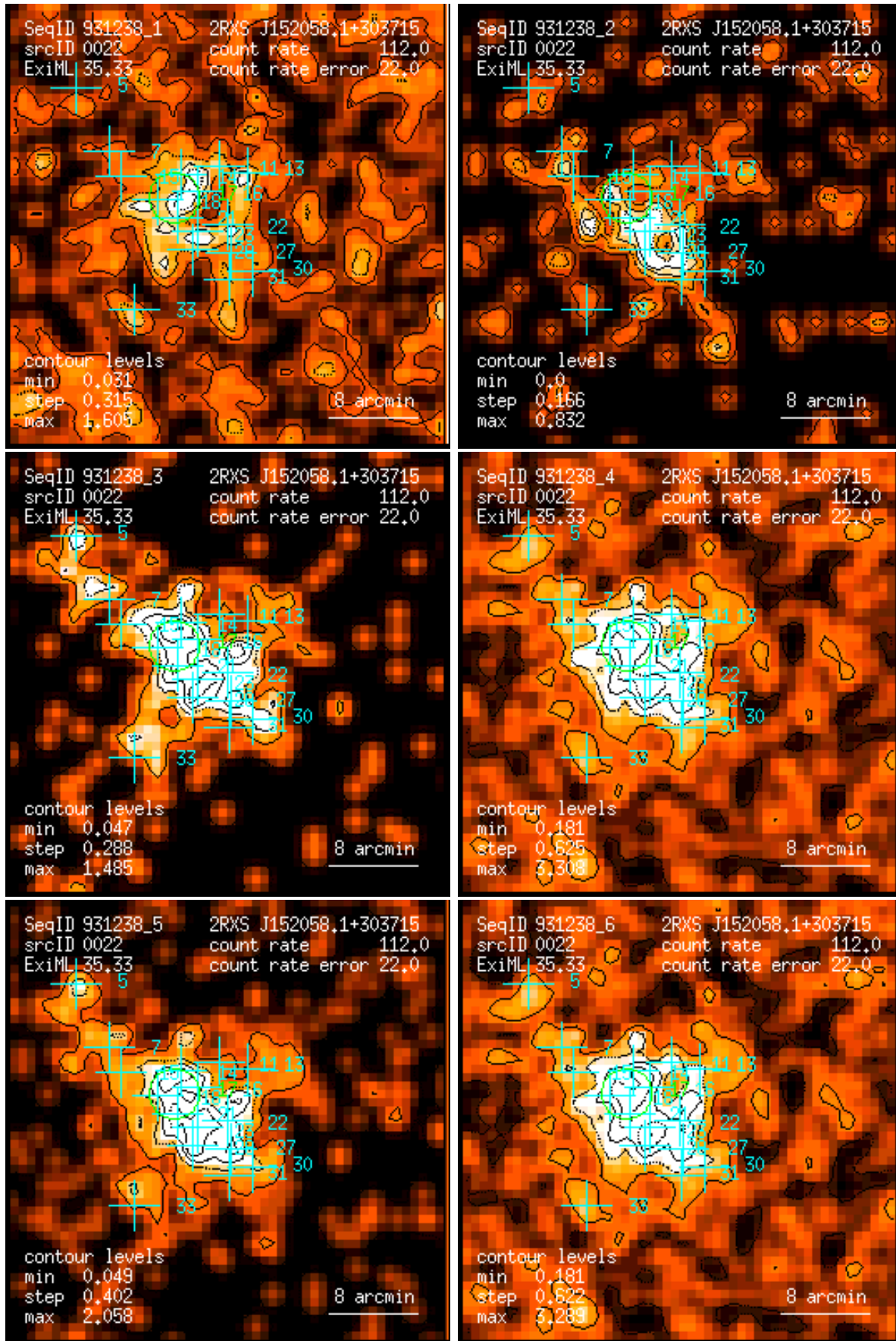
Figure 22: RASS 931238: detection 0022: band rate images, Gaussian filter: (1) PSPC channels 11 – 41, (2) 52 – 90, (3) 91 – 201, (4) 11 – 235, (5) 52 – 201, (6) 11 – 201. Broad band rates in counts/ks. Band rate contour levels in counts/ks/arcmin 2 .
