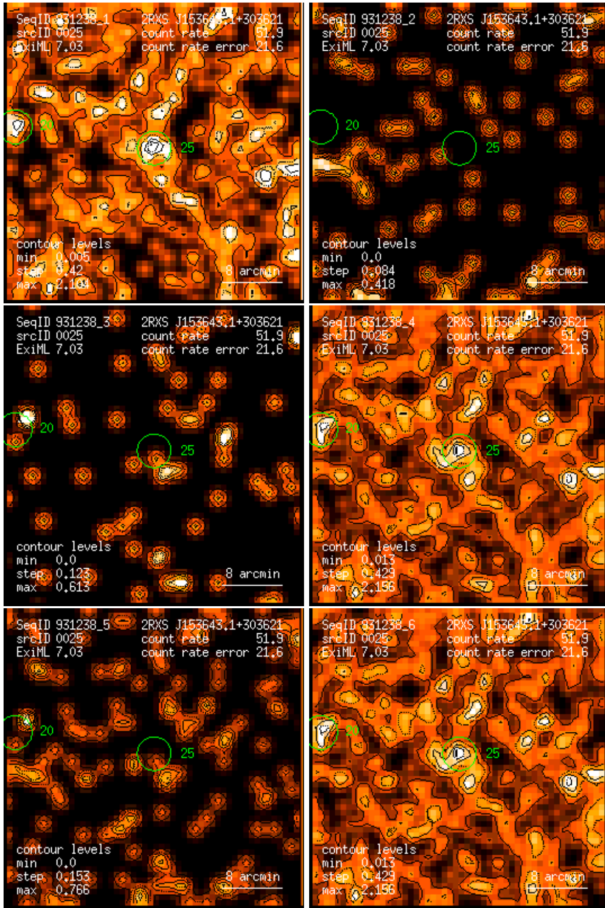
Figure 25: RASS 931238: detection 0025: band rate images, Gaussian filter: (1) PSPC channels 11 – 41, (2) 52 – 90, (3) 91 – 201, (4) 11 – 235, (5) 52 – 201, (6) 11 – 201. Broad band rates in counts/ks. Band rate contour levels in counts/ks/arcmin 2 .
