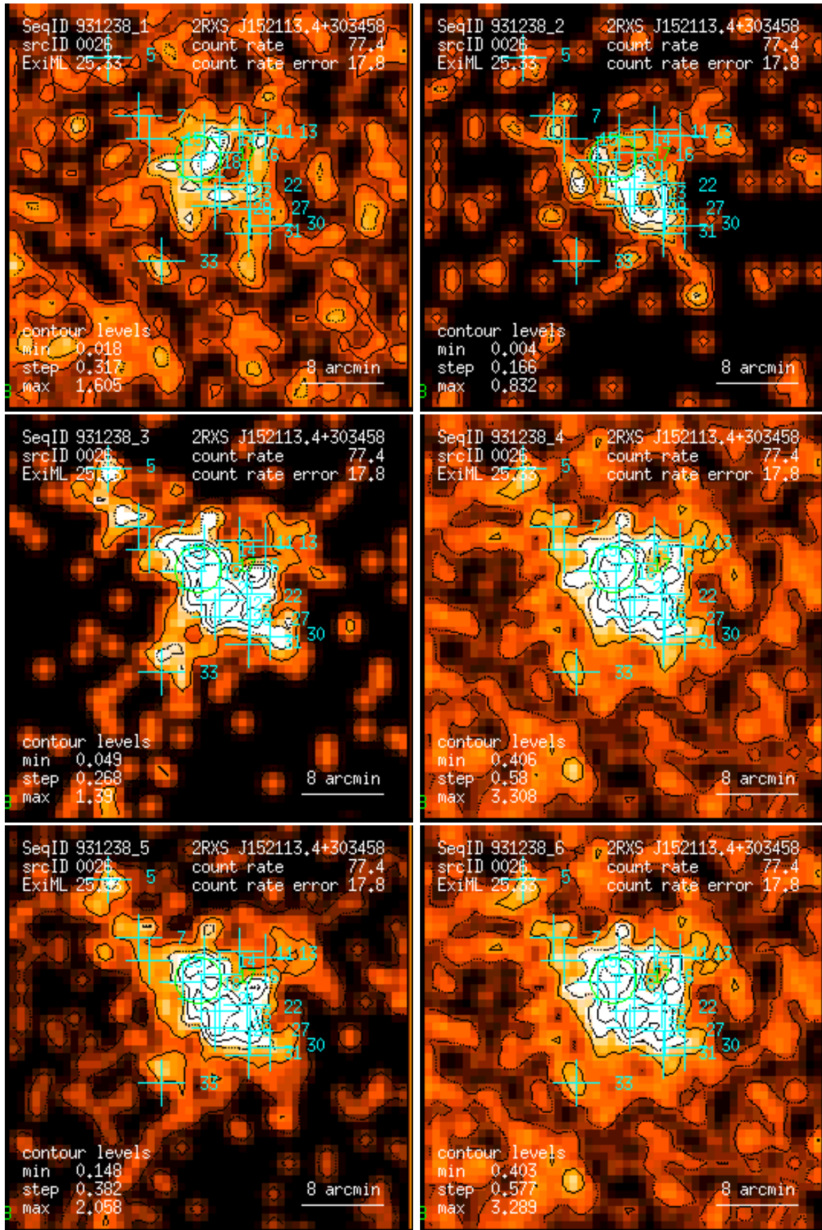
Figure 26: RASS 931238: detection 0026: band rate images, Gaussian filter: (1) PSPC channels 11 – 41, (2) 52 – 90, (3) 91 – 201, (4) 11 – 235, (5) 52 – 201, (6) 11 – 201. Broad band rates in counts/ks. Band rate contour levels in counts/ks/arcmin 2 .
