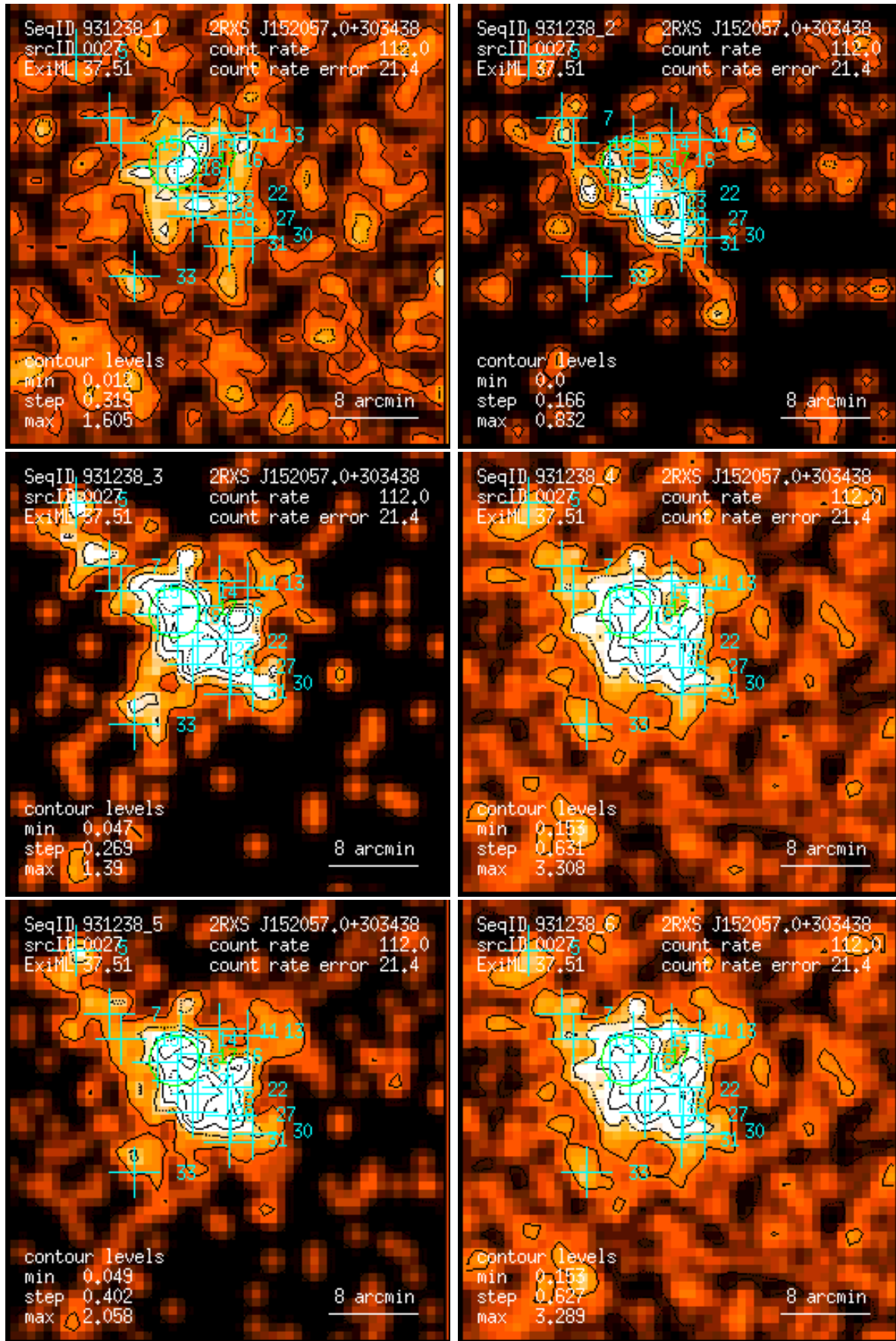
Figure 27: RASS 931238: detection 0027: band rate images, Gaussian filter: (1) PSPC channels 11 – 41, (2) 52 – 90, (3) 91 – 201, (4) 11 – 235, (5) 52 – 201, (6) 11 – 201. Broad band rates in counts/ks. Band rate contour levels in counts/ks/arcmin 2 .
