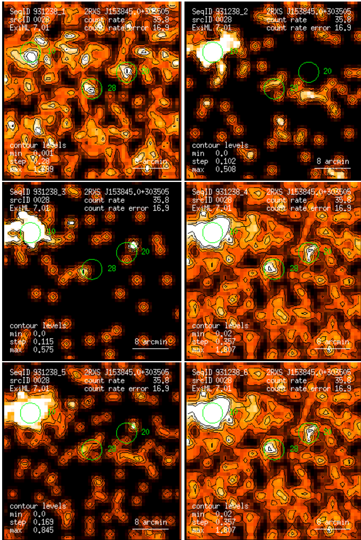
Figure 28: RASS 931238: detection 0028: band rate images, Gaussian filter: (1) PSPC channels 11 – 41, (2) 52 – 90, (3) 91 – 201, (4) 11 – 235, (5) 52 – 201, (6) 11 – 201. Broad band rates in counts/ks. Band rate contour levels in counts/ks/arcmin 2 .
