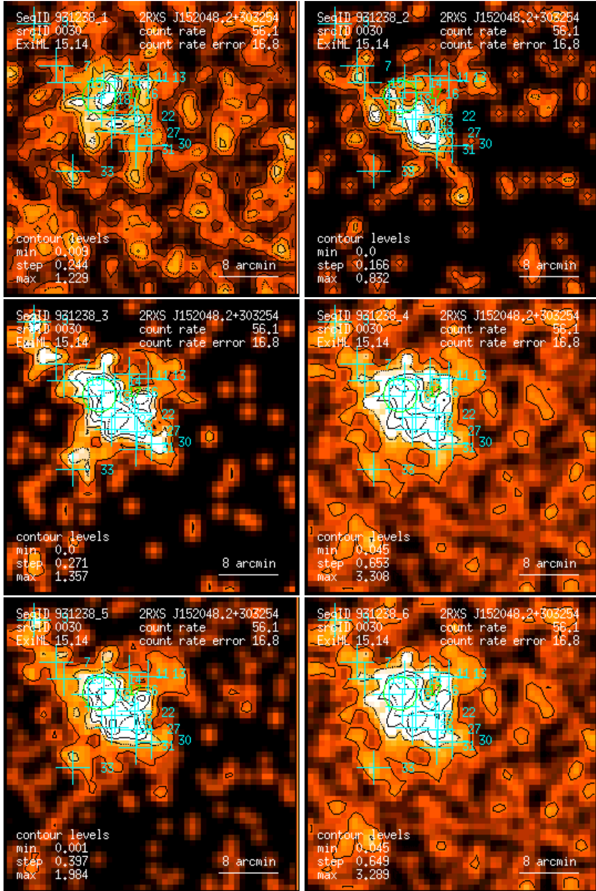
Figure 30: RASS 931238: detection 0030: band rate images, Gaussian filter: (1) PSPC channels 11 – 41, (2) 52 – 90, (3) 91 – 201, (4) 11 – 235, (5) 52 – 201, (6) 11 – 201. Broad band rates in counts/ks. Band rate contour levels in counts/ks/arcmin 2 .
