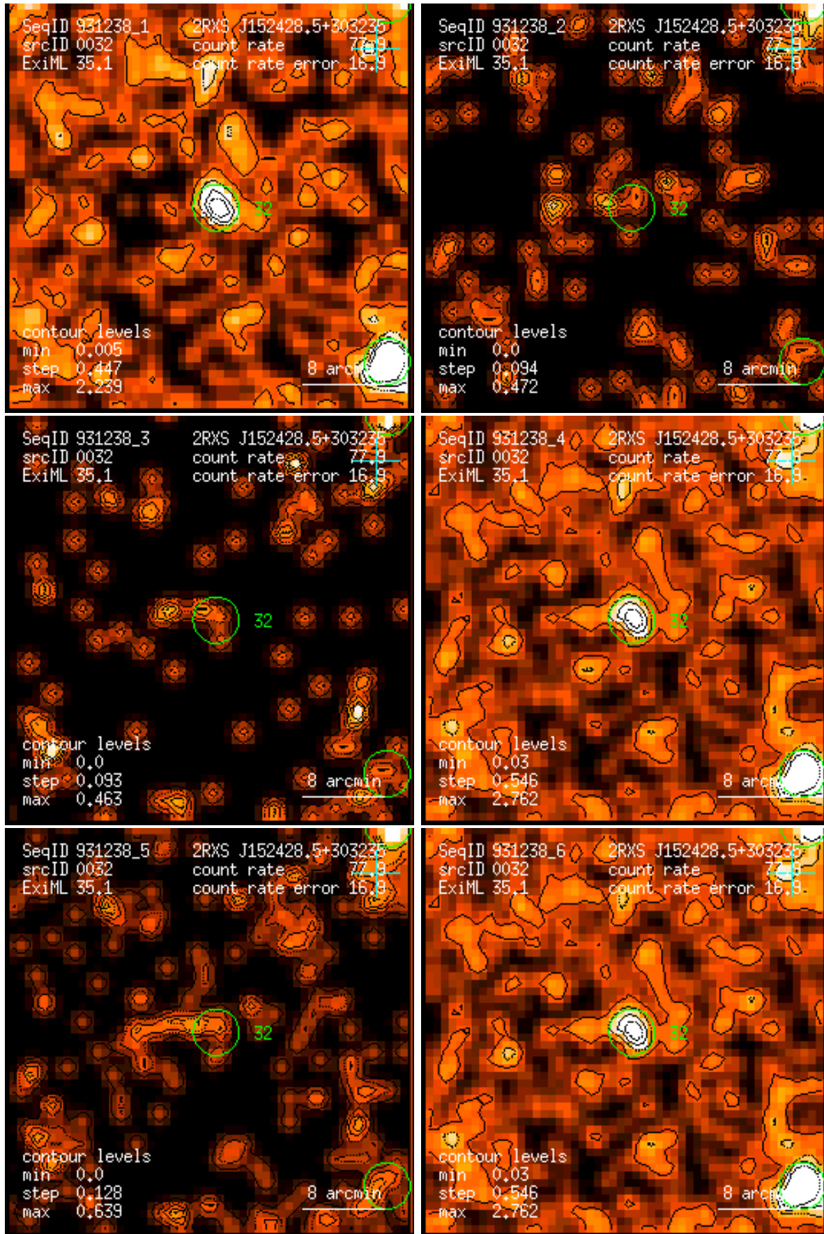
Figure 32: RASS 931238: detection 0032: band rate images, Gaussian filter: (1) PSPC channels 11 – 41, (2) 52 – 90, (3) 91 – 201, (4) 11 – 235, (5) 52 – 201, (6) 11 – 201. Broad band rates in counts/ks. Band rate contour levels in counts/ks/arcmin 2 .
