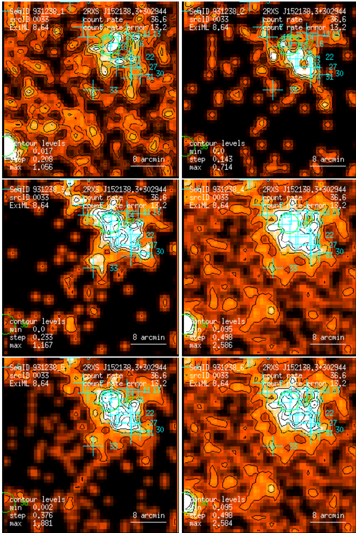
Figure 33: RASS 931238: detection 0033: band rate images, Gaussian filter: (1) PSPC channels 11 – 41, (2) 52 – 90, (3) 91 – 201, (4) 11 – 235, (5) 52 – 201, (6) 11 – 201. Broad band rates in counts/ks. Band rate contour levels in counts/ks/arcmin 2 .
