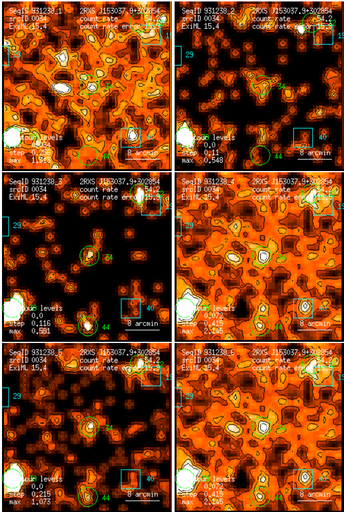
Figure 34: RASS 931238: detection 0034: band rate images, Gaussian filter: (1) PSPC channels 11 – 41, (2) 52 – 90, (3) 91 – 201, (4) 11 – 235, (5) 52 – 201, (6) 11 – 201. Broad band rates in counts/ks. Band rate contour levels in counts/ks/arcmin 2 .
