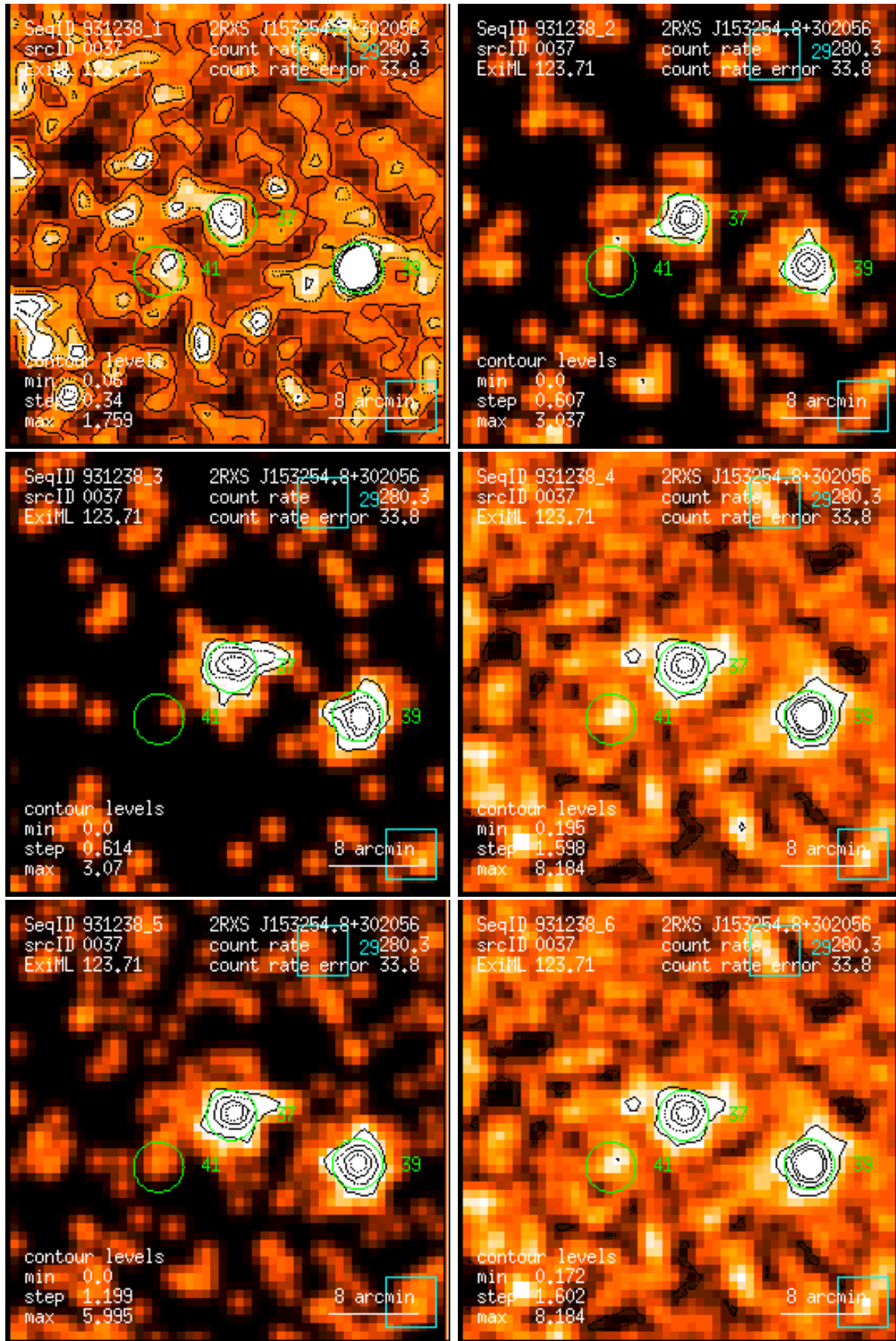
Figure 37: RASS 931238: detection 0037: band rate images, Gaussian filter: (1) PSPC channels 11 – 41, (2) 52 – 90, (3) 91 – 201, (4) 11 – 235, (5) 52 – 201, (6) 11 – 201. Broad band rates in counts/ks. Band rate contour levels in counts/ks/arcmin 2 .
