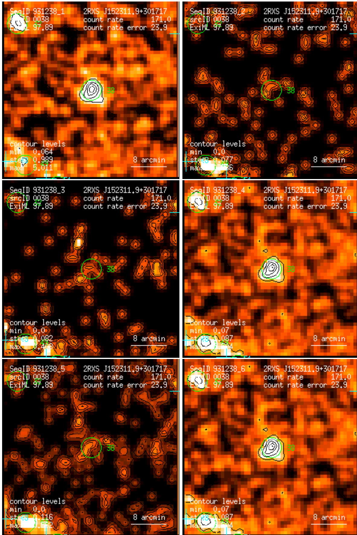
Figure 38: RASS 931238: detection 0038: band rate images, Gaussian filter: (1) PSPC channels 11 – 41, (2) 52 – 90, (3) 91 – 201, (4) 11 – 235, (5) 52 – 201, (6) 11 – 201. Broad band rates in counts/ks. Band rate contour levels in counts/ks/arcmin 2 .
