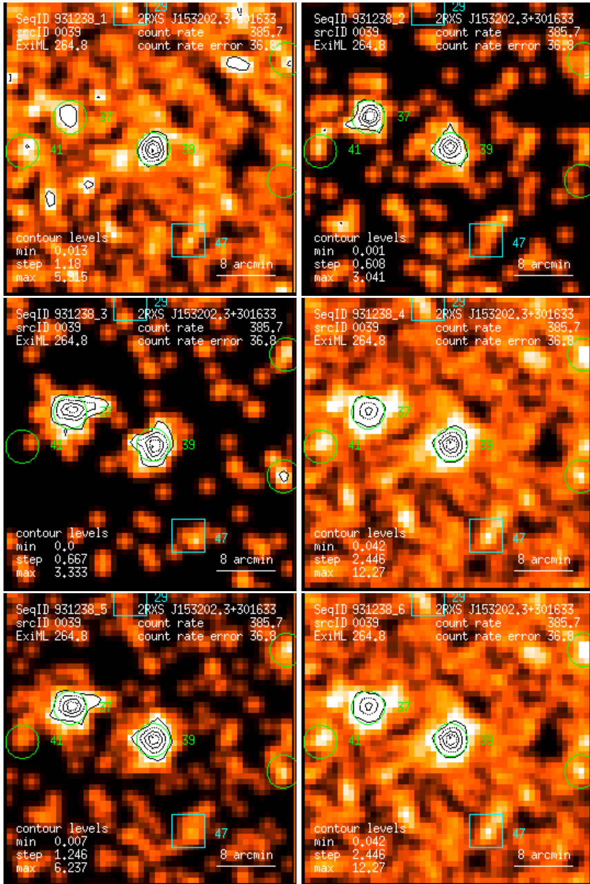
Figure 39: RASS 931238: detection 0039: band rate images, Gaussian filter: (1) PSPC channels 11 – 41, (2) 52 – 90, (3) 91 – 201, (4) 11 – 235, (5) 52 – 201, (6) 11 – 201. Broad band rates in counts/ks. Band rate contour levels in counts/ks/arcmin 2 .
