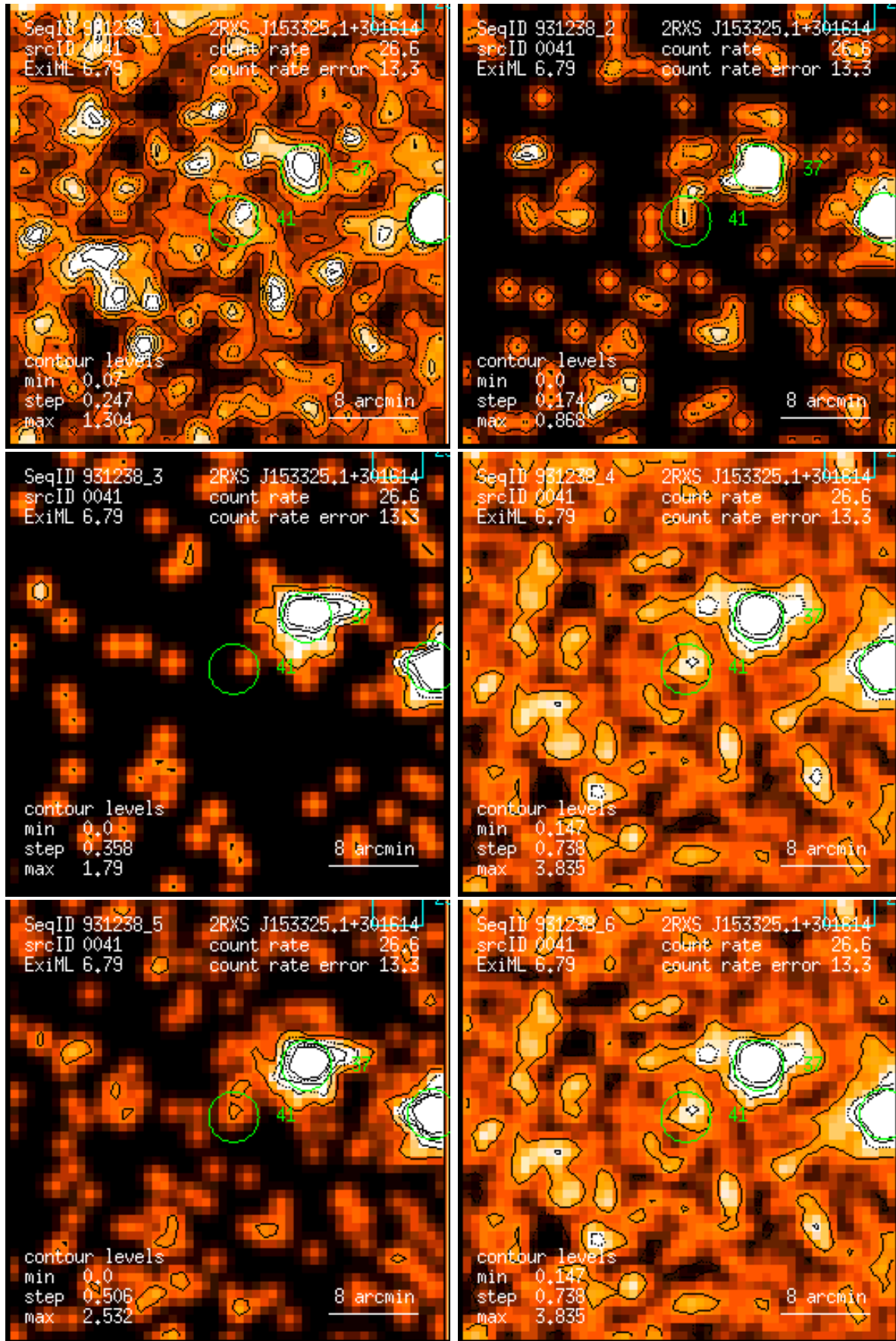
Figure 41: RASS 931238: detection 0041: band rate images, Gaussian filter: (1) PSPC channels 11 – 41, (2) 52 – 90, (3) 91 – 201, (4) 11 – 235, (5) 52 – 201, (6) 11 – 201. Broad band rates in counts/ks. Band rate contour levels in counts/ks/arcmin 2 .
