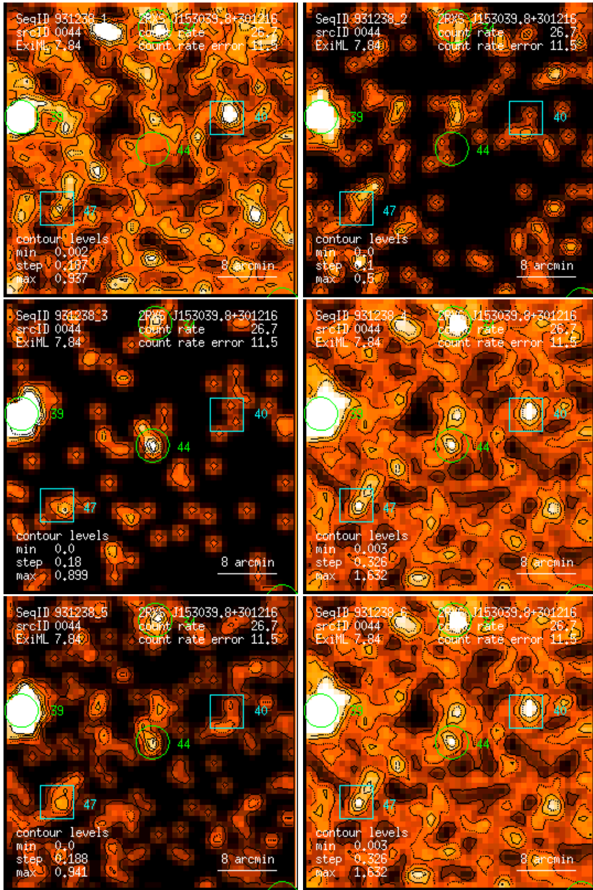
Figure 44: RASS 931238: detection 0044: band rate images, Gaussian filter: (1) PSPC channels 11 – 41, (2) 52 – 90, (3) 91 – 201, (4) 11 – 235, (5) 52 – 201, (6) 11 – 201. Broad band rates in counts/ks. Band rate contour levels in counts/ks/arcmin 2 .
