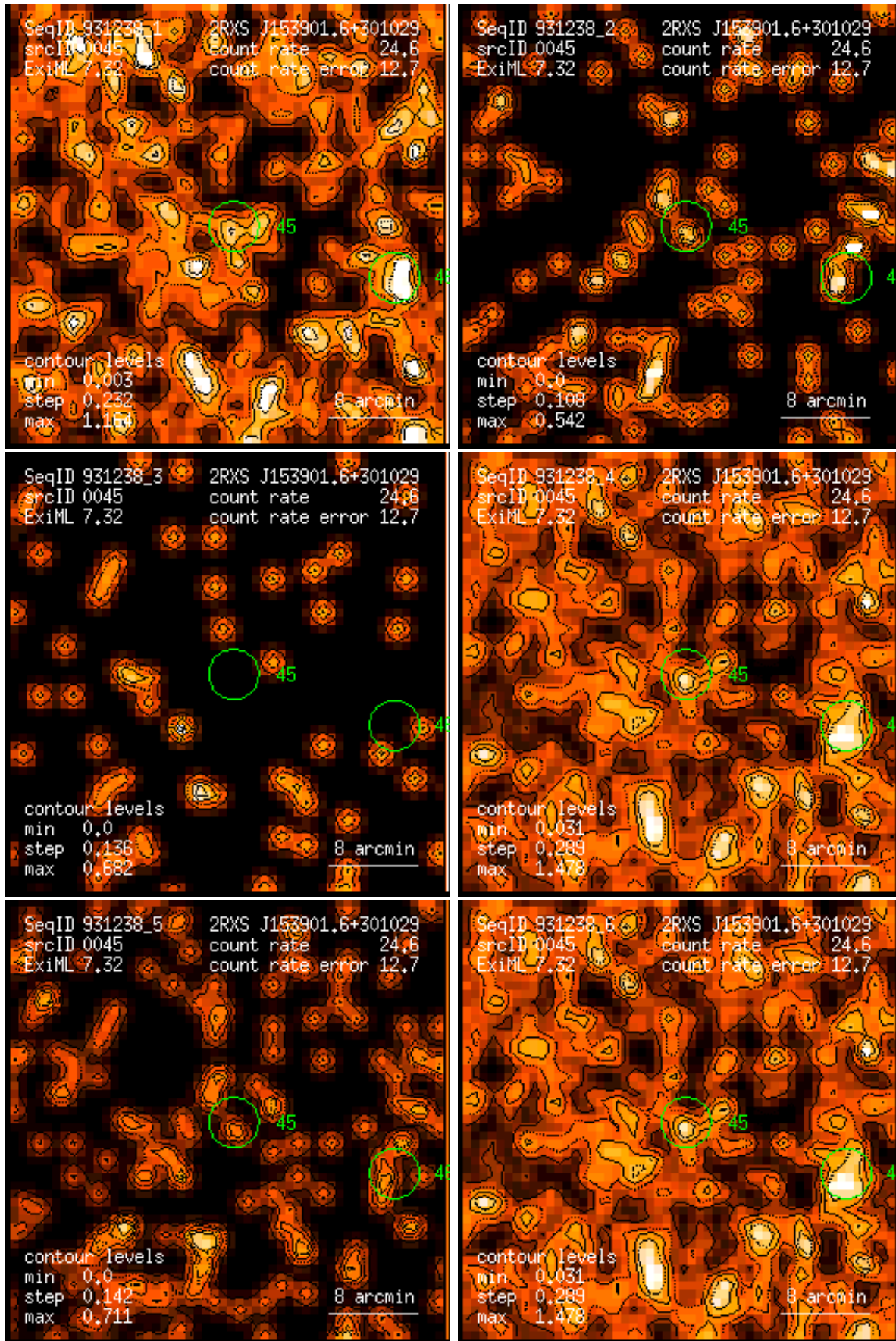
Figure 45: RASS 931238: detection 0045: band rate images, Gaussian filter: (1) PSPC channels 11 – 41, (2) 52 – 90, (3) 91 – 201, (4) 11 – 235, (5) 52 – 201, (6) 11 – 201. Broad band rates in counts/ks. Band rate contour levels in counts/ks/arcmin 2 .
