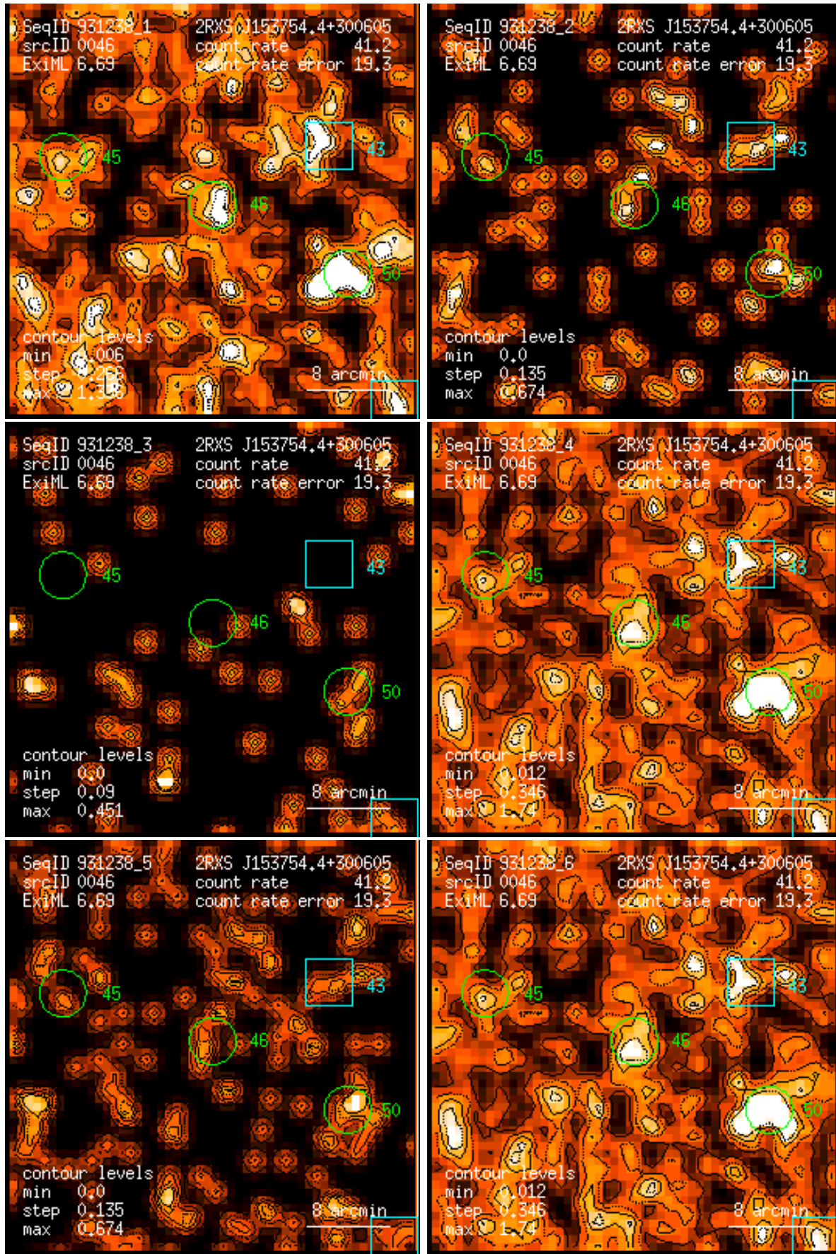
Figure 46: RASS 931238: detection 0046: band rate images, Gaussian filter: (1) PSPC channels 11 – 41, (2) 52 – 90, (3) 91 – 201, (4) 11 – 235, (5) 52 – 201, (6) 11 – 201. Broad band rates in counts/ks. Band rate contour levels in counts/ks/arcmin 2 .
