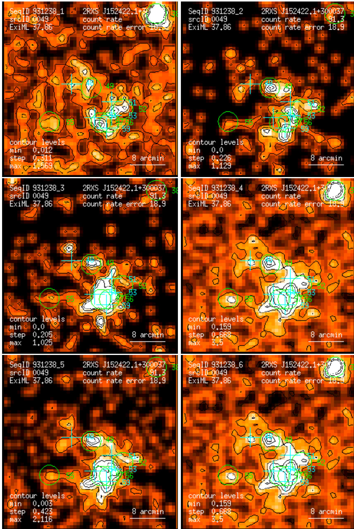
Figure 49: RASS 931238: detection 0049: band rate images, Gaussian filter: (1) PSPC channels 11 – 41, (2) 52 – 90, (3) 91 – 201, (4) 11 – 235, (5) 52 – 201, (6) 11 – 201. Broad band rates in counts/ks. Band rate contour levels in counts/ks/arcmin 2 .
