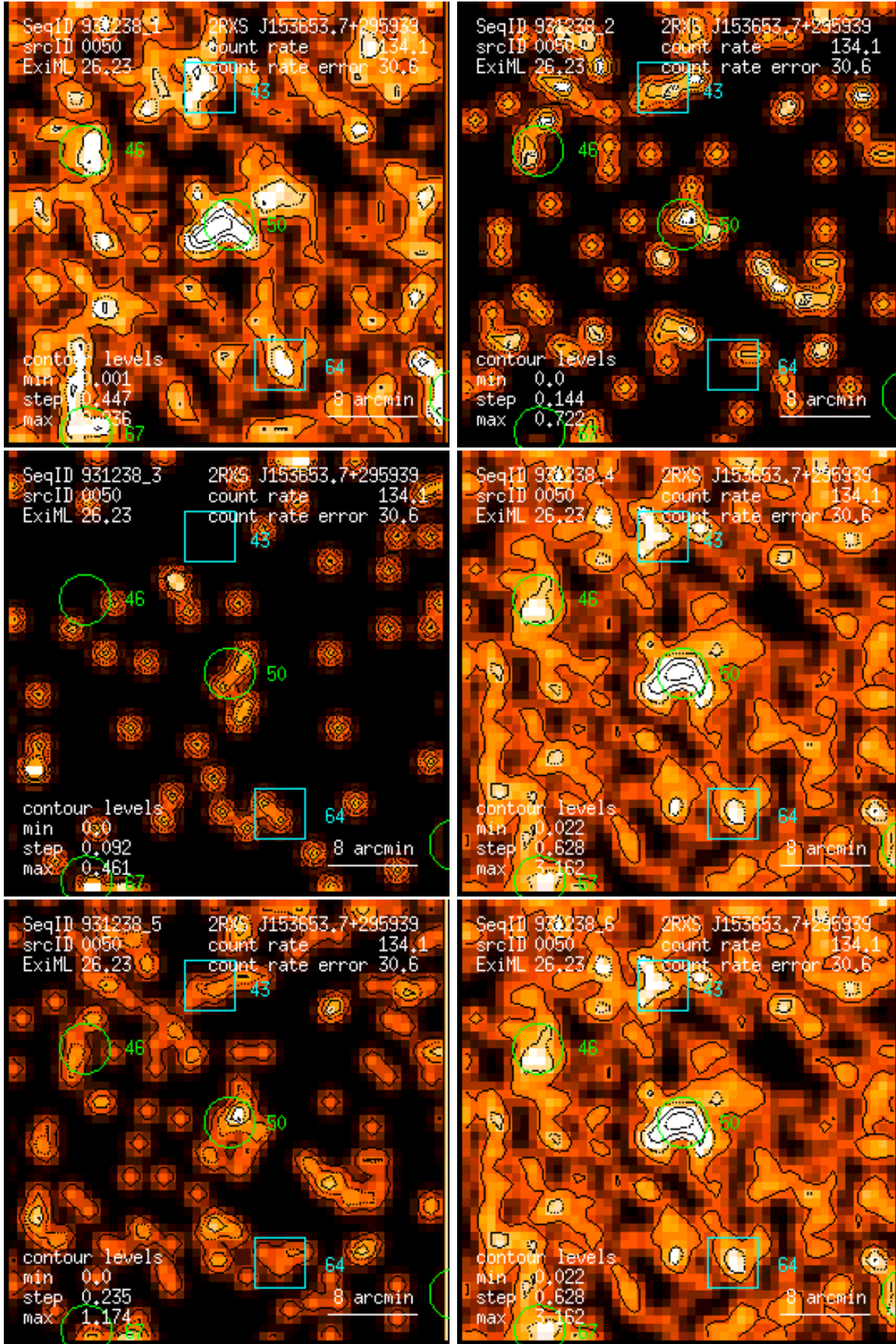
Figure 50: RASS 931238: detection 0050: band rate images, Gaussian filter: (1) PSPC channels 11 – 41, (2) 52 – 90, (3) 91 – 201, (4) 11 – 235, (5) 52 – 201, (6) 11 – 201. Broad band rates in counts/ks. Band rate contour levels in counts/ks/arcmin 2 .
