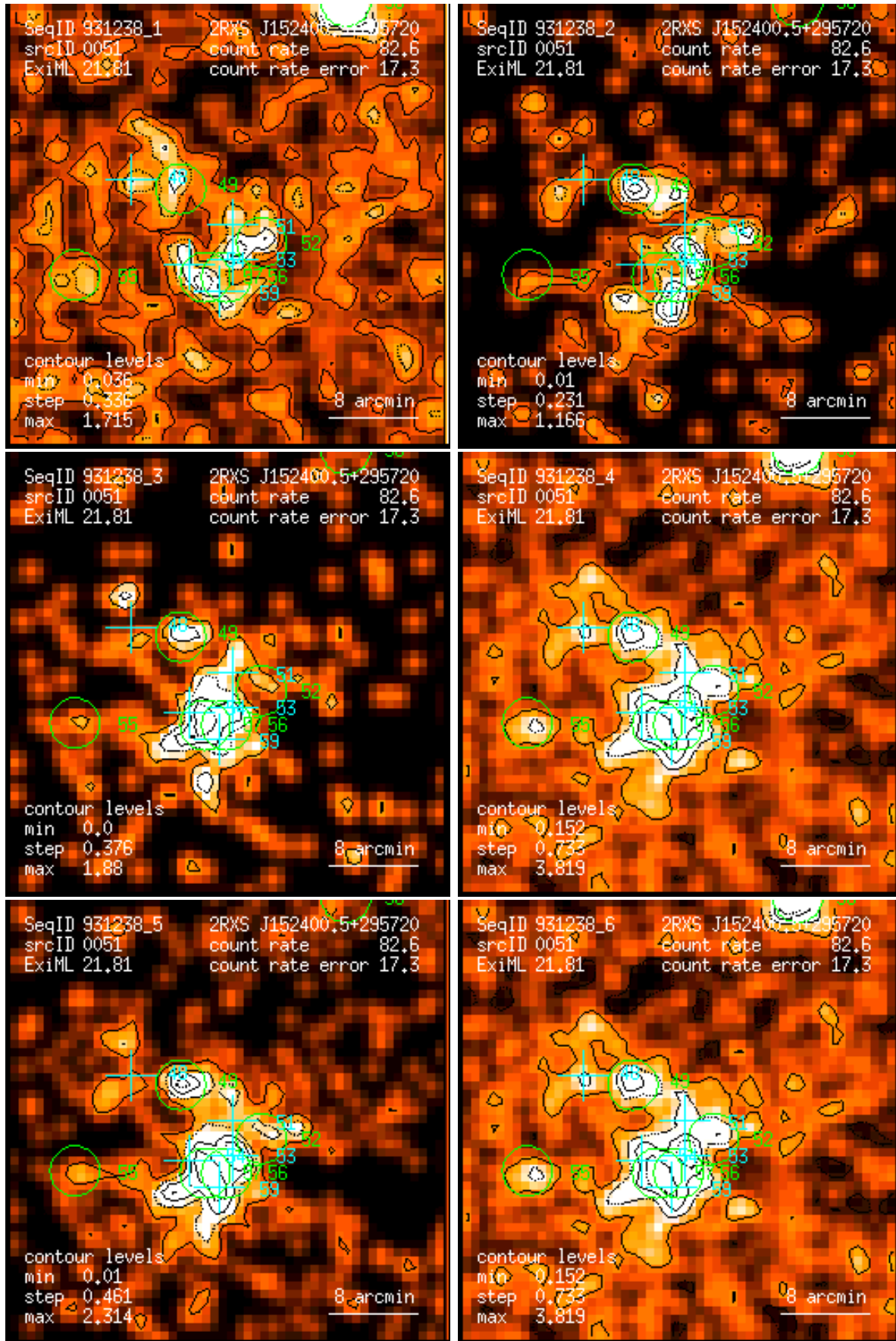
Figure 51: RASS 931238: detection 0051: band rate images, Gaussian filter: (1) PSPC channels 11 – 41, (2) 52 – 90, (3) 91 – 201, (4) 11 – 235, (5) 52 – 201, (6) 11 – 201. Broad band rates in counts/ks. Band rate contour levels in counts/ks/arcmin 2 .
