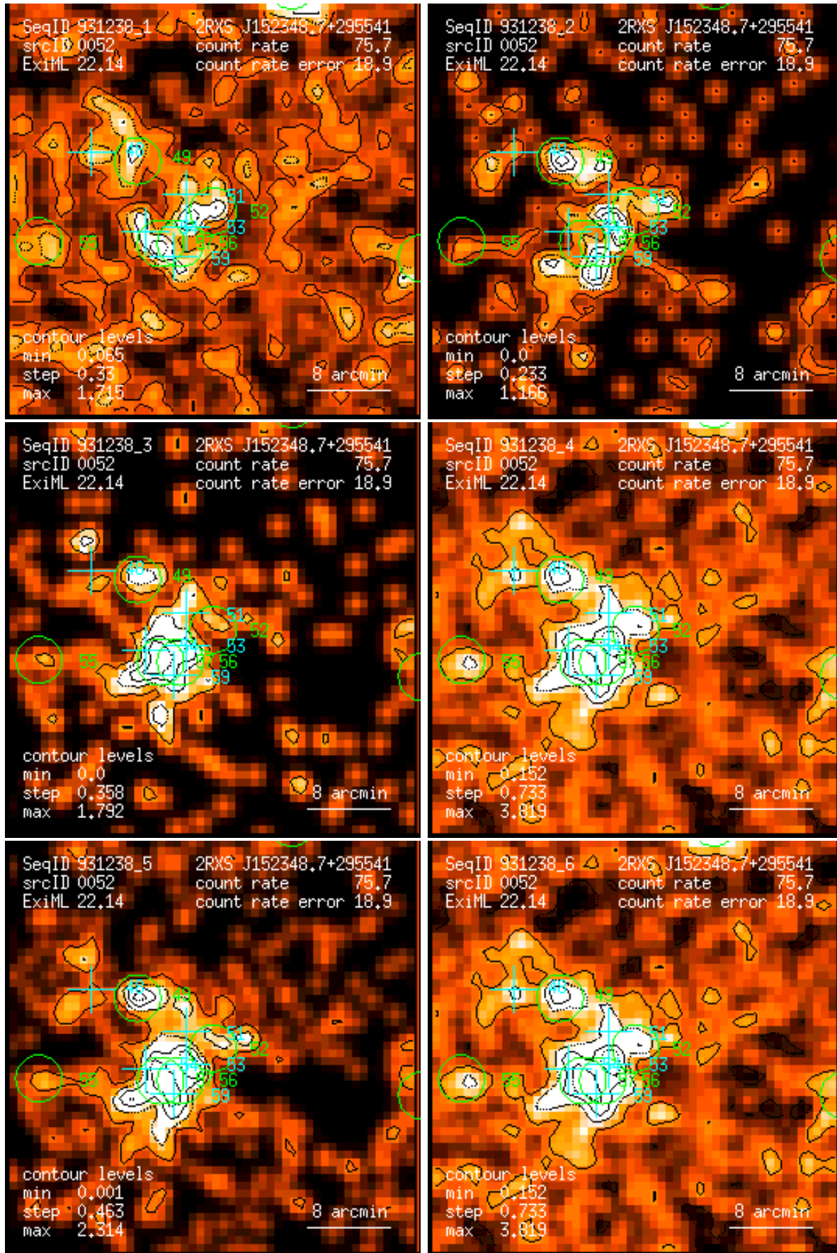
Figure 52: RASS 931238: detection 0052: band rate images, Gaussian filter: (1) PSPC channels 11 – 41, (2) 52 – 90, (3) 91 – 201, (4) 11 – 235, (5) 52 – 201, (6) 11 – 201. Broad band rates in counts/ks. Band rate contour levels in counts/ks/arcmin 2 .
