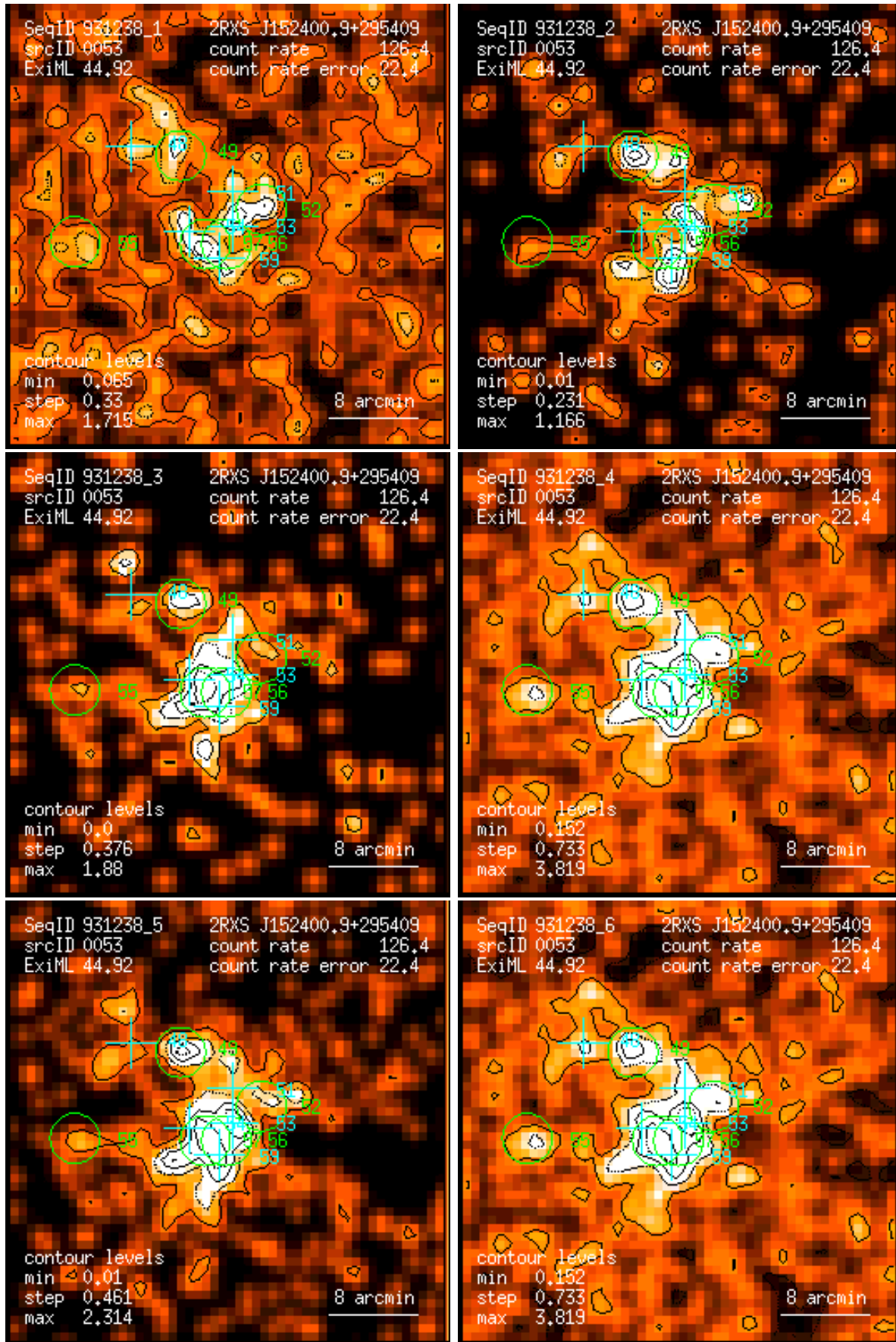
Figure 53: RASS 931238: detection 0053: band rate images, Gaussian filter: (1) PSPC channels 11 – 41, (2) 52 – 90, (3) 91 – 201, (4) 11 – 235, (5) 52 – 201, (6) 11 – 201. Broad band rates in counts/ks. Band rate contour levels in counts/ks/arcmin 2 .
