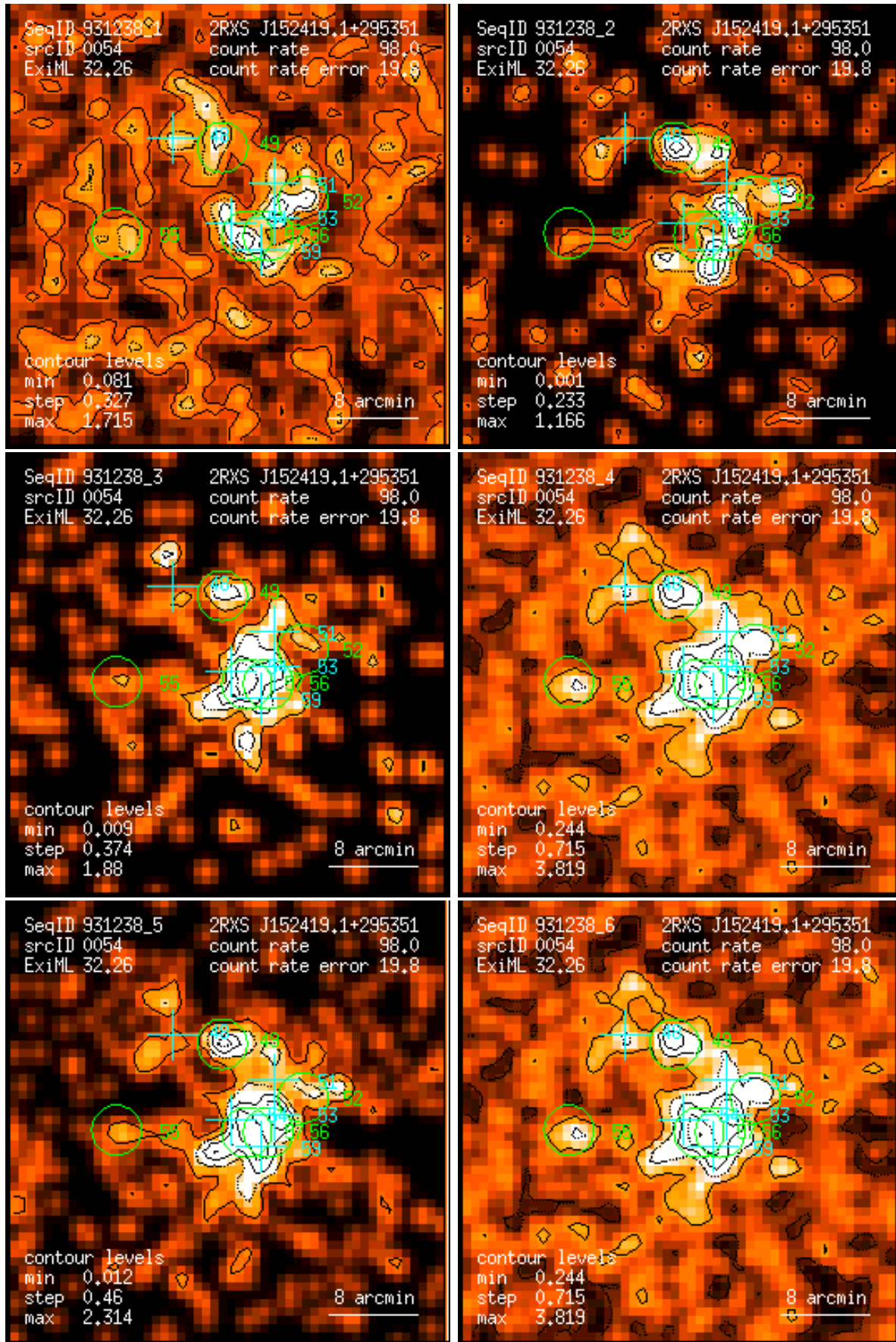
Figure 54: RASS 931238: detection 0054: band rate images, Gaussian filter: (1) PSPC channels 11 – 41, (2) 52 – 90, (3) 91 – 201, (4) 11 – 235, (5) 52 – 201, (6) 11 – 201. Broad band rates in counts/ks. Band rate contour levels in counts/ks/arcmin 2 .
