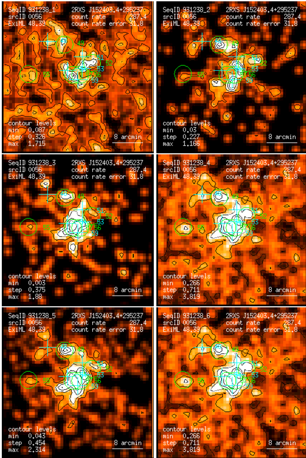
Figure 56: RASS 931238: detection 0056: band rate images, Gaussian filter: (1) PSPC channels 11 – 41, (2) 52 – 90, (3) 91 – 201, (4) 11 – 235, (5) 52 – 201, (6) 11 – 201. Broad band rates in counts/ks. Band rate contour levels in counts/ks/arcmin 2 .
