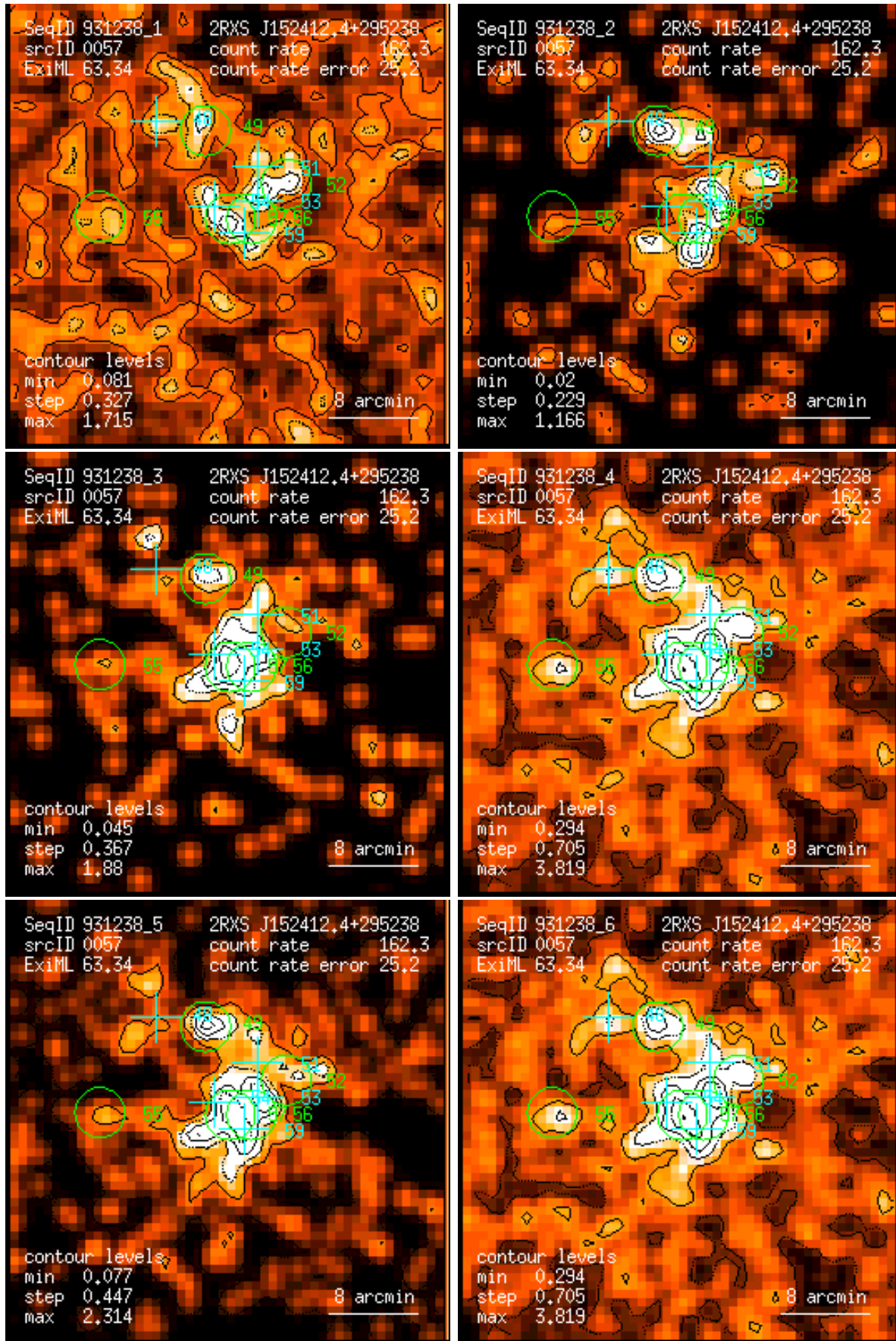
Figure 57: RASS 931238: detection 0057: band rate images, Gaussian filter: (1) PSPC channels 11 – 41, (2) 52 – 90, (3) 91 – 201, (4) 11 – 235, (5) 52 – 201, (6) 11 – 201. Broad band rates in counts/ks. Band rate contour levels in counts/ks/arcmin 2 .
