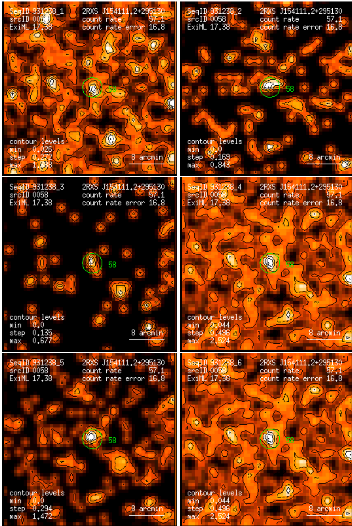
Figure 58: RASS 931238: detection 0058: band rate images, Gaussian filter: (1) PSPC channels 11 – 41, (2) 52 – 90, (3) 91 – 201, (4) 11 – 235, (5) 52 – 201, (6) 11 – 201. Broad band rates in counts/ks. Band rate contour levels in counts/ks/arcmin 2 .
