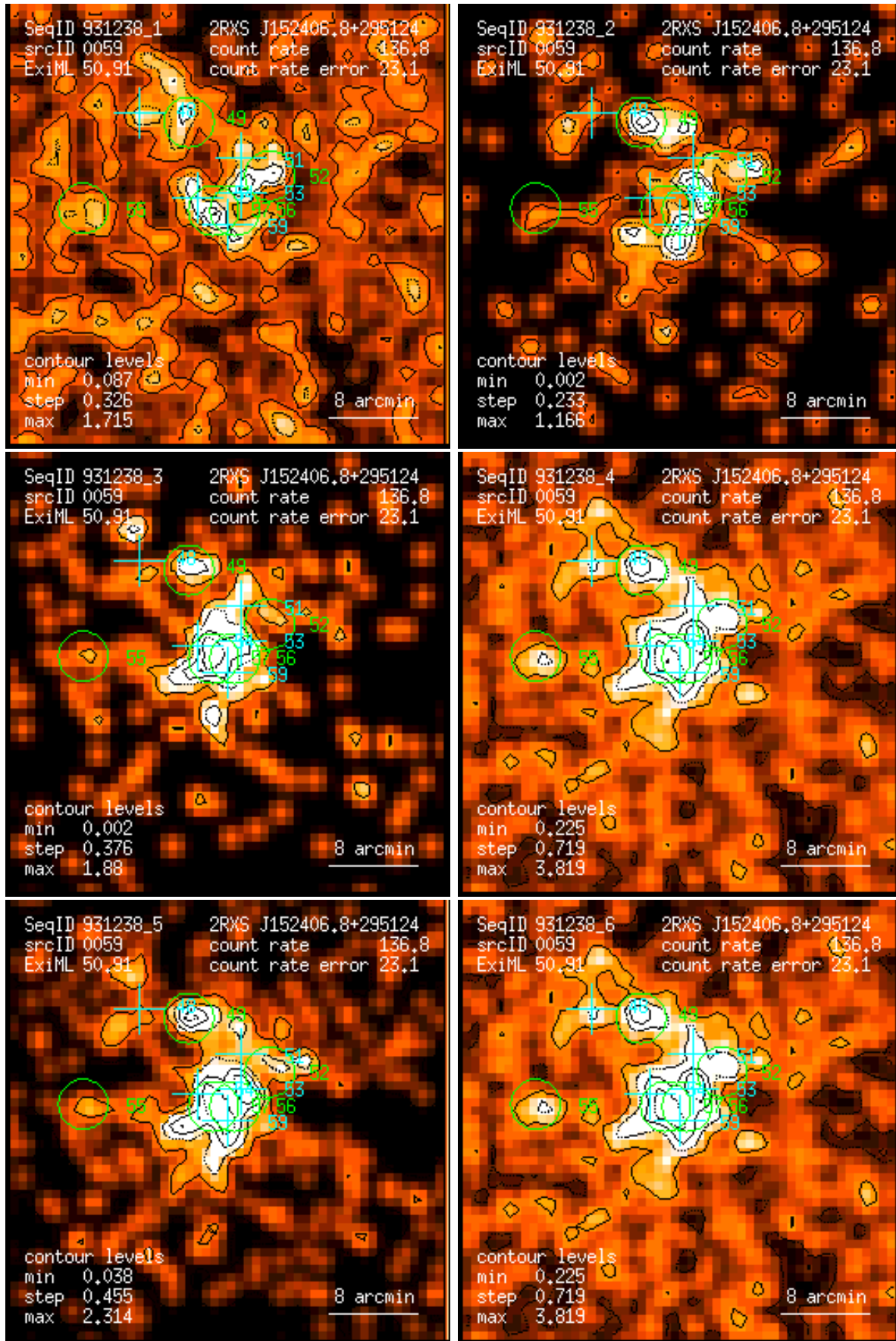
Figure 59: RASS 931238: detection 0059: band rate images, Gaussian filter: (1) PSPC channels 11 – 41, (2) 52 – 90, (3) 91 – 201, (4) 11 – 235, (5) 52 – 201, (6) 11 – 201. Broad band rates in counts/ks. Band rate contour levels in counts/ks/arcmin 2 .
